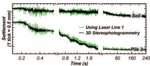
Fig. 7. Comparison of soil (at marker S3-2) and pile 2 settlement obtained from the processing of laser line 1 with measurements from 3D stereophotogrammetry.
