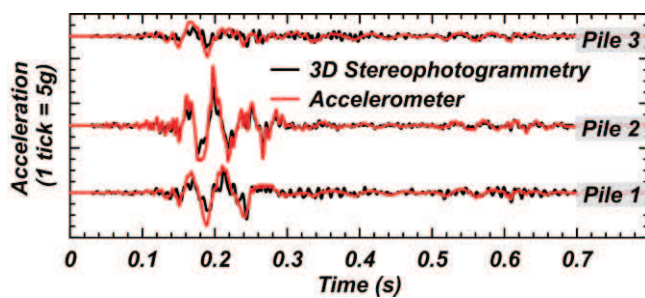
Fig. 5. Comparison of acceleration in piles obtained from 3D stereophotogrammetry with measurements from accelerometers for shaking event EQM 5 .
