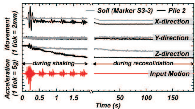
Fig. 3. 3D movement of pile 2 and soil nearby (marker S3-3) during shaking event EQM5.
