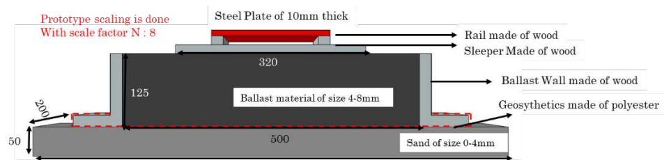
Figure 3. Illustration of the test setup (dimensions in mm)
