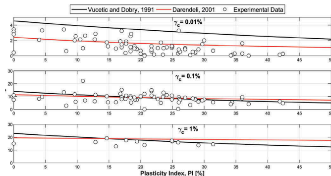
Figure 6. Variation of D vs PI for fixed \gamma_c values: 0.01%, 0.1%, and 1%.
