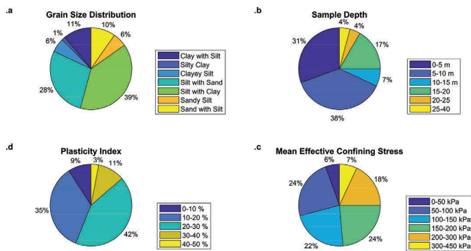
Figure 2. Characteristics of the samples: .a grain size distribution, .b sample depth, .c PI , and .d \sigma'_m .
