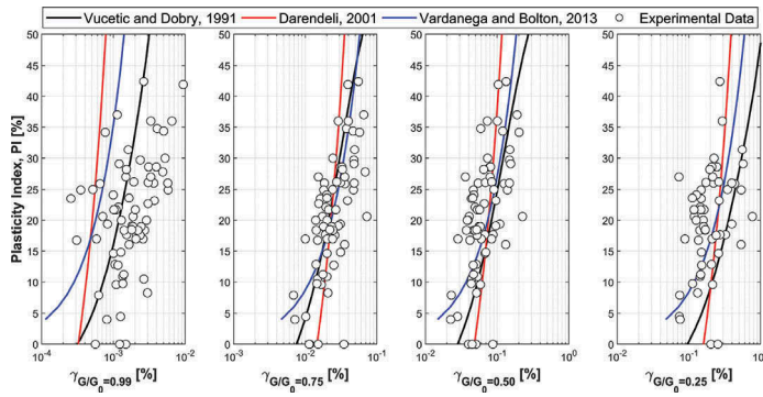
Figure 5. Variation of \gamma_c vs PI for fixed G/G_0 values: 0.99, 0.75, 0.5, and 0.25.
