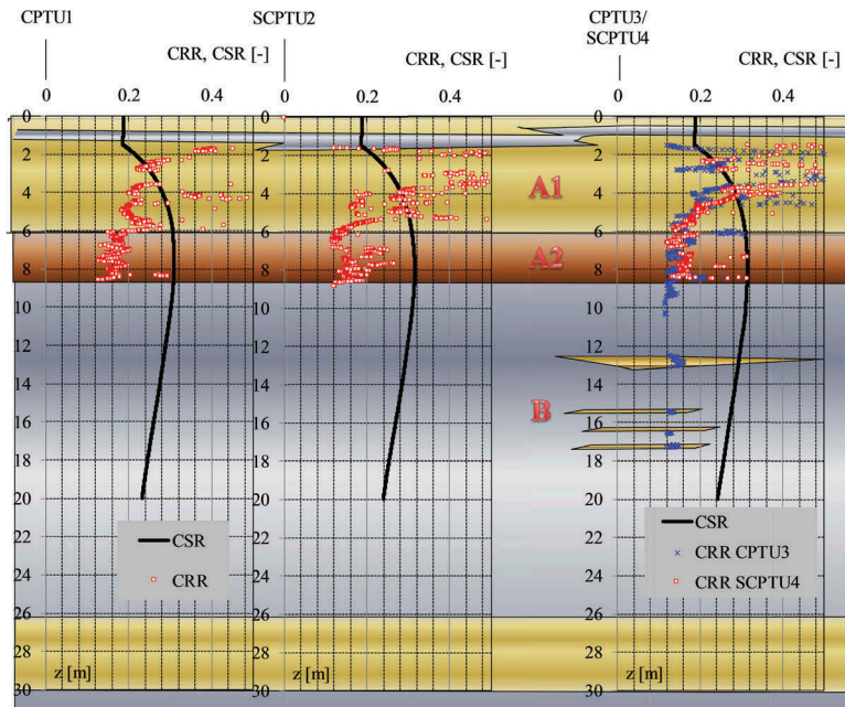
Figure 4. Soil cyclic resistance ratio CRR and earthquake induced stress ratio CSR as a function of depth, according to Idriss and Boulanger (2008).
