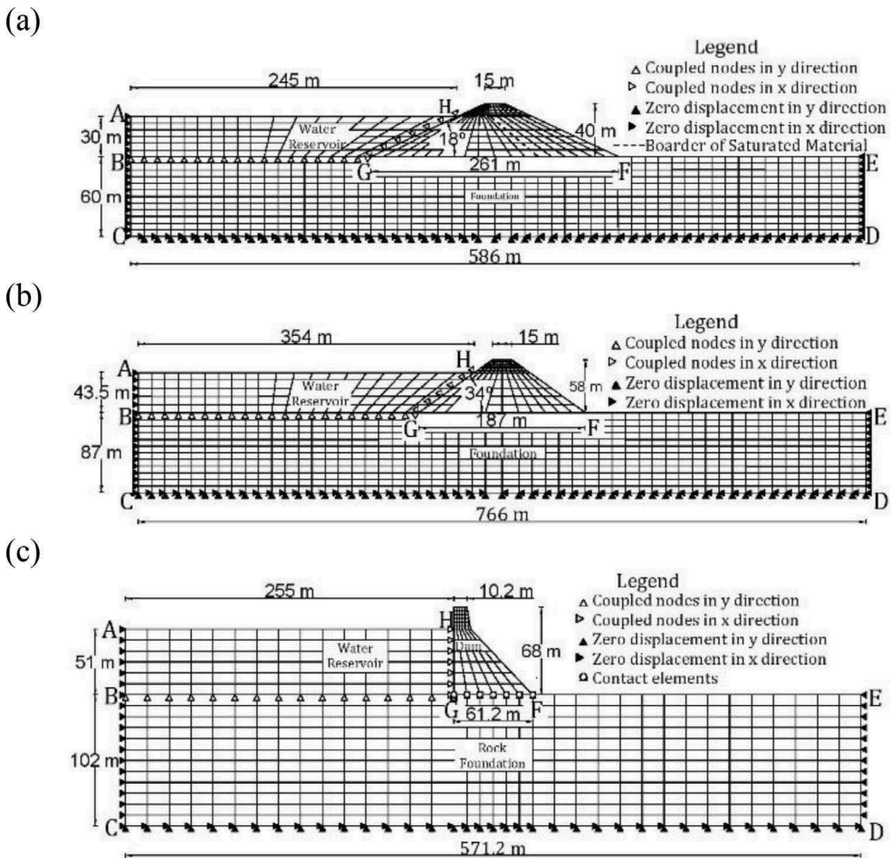
Figure 1. Finite element model geometry of a) earth dam b) rockfill dam c) concrete gravity dam
