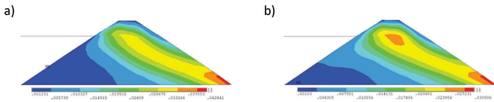
Figure 3. Von Mises strains in rockfill dam body: a) Kobe earthquake b) San Fernando earthquake
