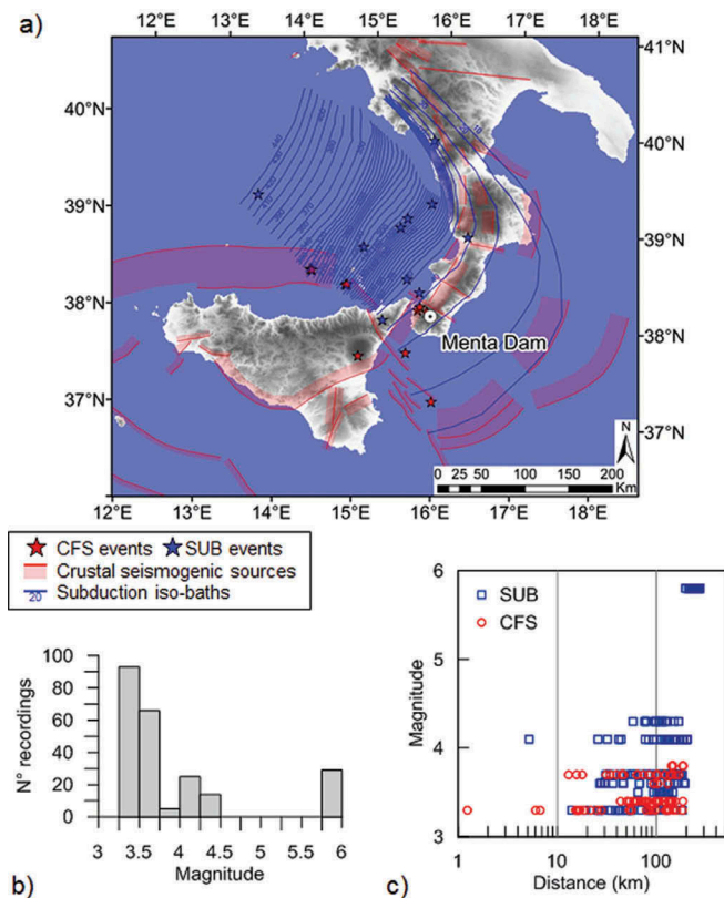
Figure 1. a) Sketch map that illustrates the main tectonic features of the study area (from DISS database, DISS Working group 2018) and the n.20 events considered for the present study; b) and c) characteristics of the recording database in terms of magnitude and distance. CFS: crustal fault source, SUB: subduction.
