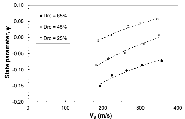
Figure 7: V_s versus state parameter ( \psi ) from the DSS tests of this study
