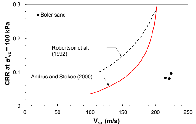
Figure 13. Comparison of CRR_1 (at \sigma'_{vc} = 100 kPa) and V_{S1} for Boler sand with liquefaction triggering curves of Andrus and Stokoe (2000) and Robertson et al. (1992)
