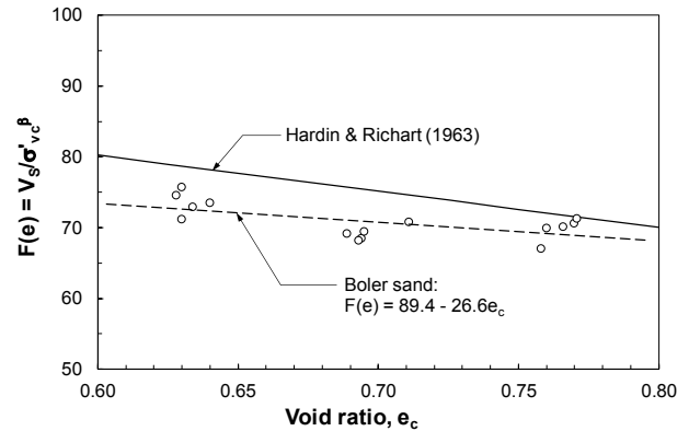
Figure 6. Variation of F(e) with consolidation void ratio ( e_c ) from the experiments of this study for Boler and comparison with the correlation derived by Hardin and Richart (1963)
