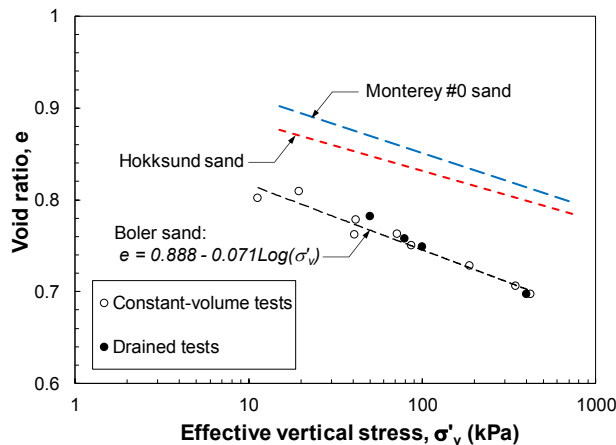
Figure 3. Critical state lines of Boler (from this study), Hokksund (Castro, 1969), and Monterey #0 (Jefferies and Been, 2006) sands
