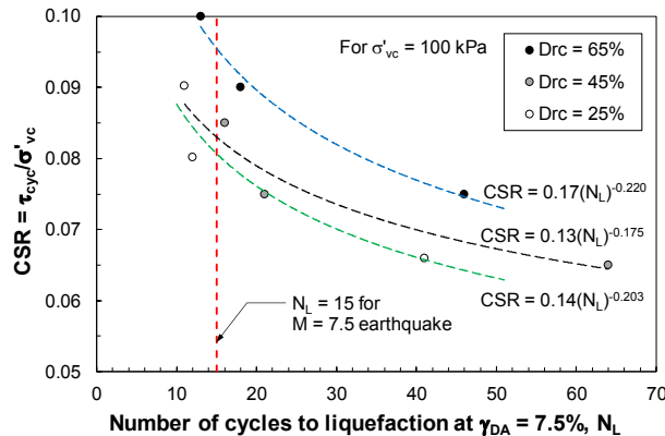
Figure 12. CSR versus number of cycles ( N_L ) to trigger liquefaction for Boler sand at \sigma'_{vc} = 100 kPa
