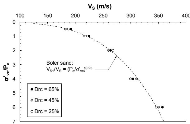
Figure 5. Variation of V_s with normalized effective vertical stress ( \sigma'_{vc}/P_a ) for Boler sand specimens
