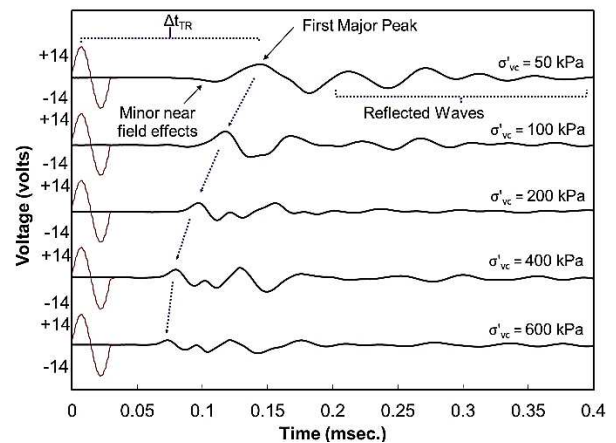
Figure 4. Shear wave signals for D_{rc} = 45\% specimen
