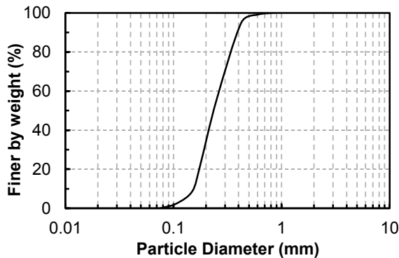
Figure 1. Average grain size distribution of Boler sand
