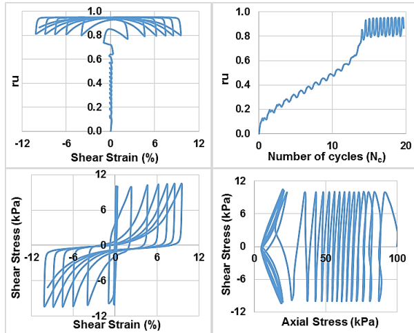
Figure 11. Cyclic DSS test results on a Boler sand specimen at D_{rc} = 65\% , \sigma'_{vc} = 100 kPa and CSR = 0.100
