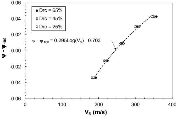
Figure 8. V_S versus (\psi - \psi_{100}) from the DSS tests of this study. \psi_{100} is the state parameter at \sigma'_{vc} = 100 kPa
