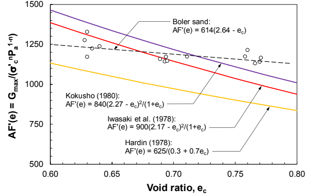
Figure 10. Variations of AF'(e) with e_c for Boler sand tested as well as those suggested by several other studies (Hardin 1978; Iwasaki et al. 1978; Kokusho 1980) for clean sands
