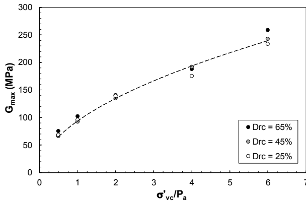
Figure 9. Variation of G_{max} with \sigma'_{vc} for Boler sand at D_{rc} = 25, 45, and 65\%
