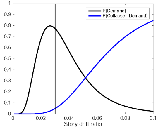
Figure 6. Illustration of assumed MCE demand and collapse capacity for the baseline base. P(Demand) is a probability density function, while P(Collapse|Demand) is a probability, conditional on the specified demand level. The mean value of the demand distribution is shown with a thin vertical line.
