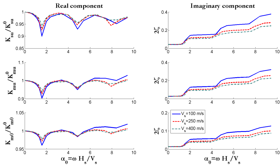
Figure 5. Variation of the three dynamic stiffness coefficients with respect to the dimensionless frequency. Effect of V_s on the real component (a) and the imaginary component (b).
