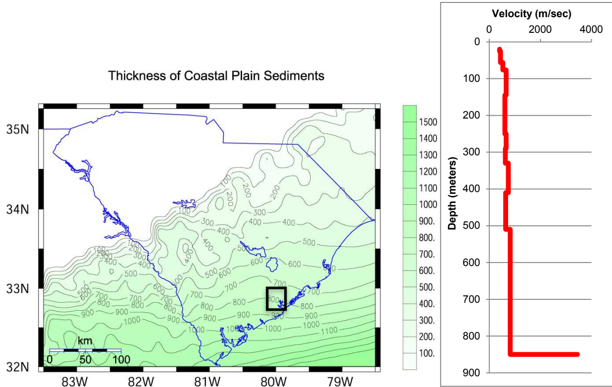
Figure 1. Left: Thickness of coastal plain sediments derived from borehole and geophysical data (Figure 6 from Chapman and Talwani, 2006; used with permission.). Black box is our study area. Right: Shear wave velocity from the top of bedrock to the base of the Tertiary section.
