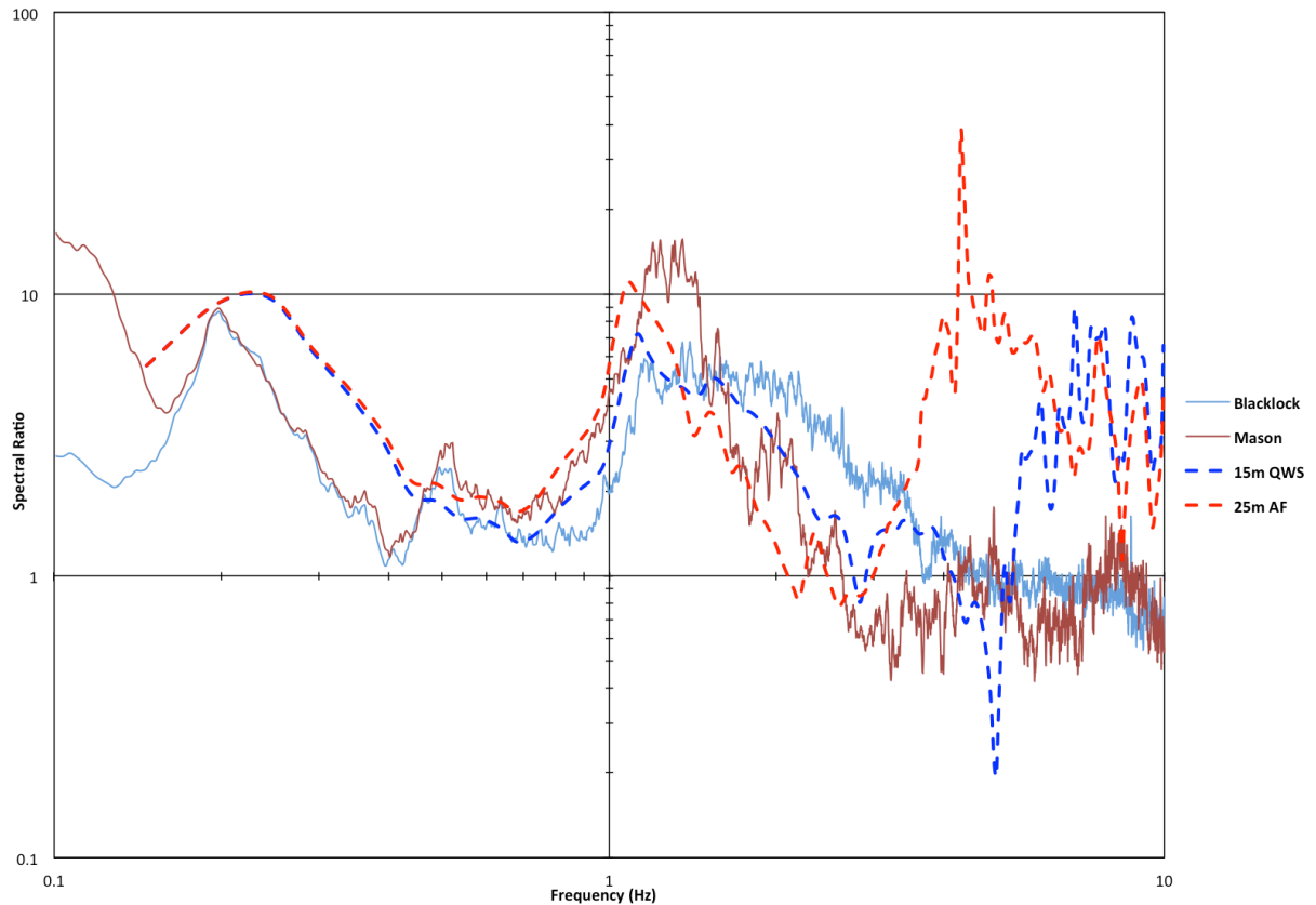
Figure 3. Observed (solid) and modeled (dashed) HVSR at 2 sites on the Charleston Peninsula. Red - site on artificial fill above marsh deposits; blue – site on Quaternary Wando Formation.
