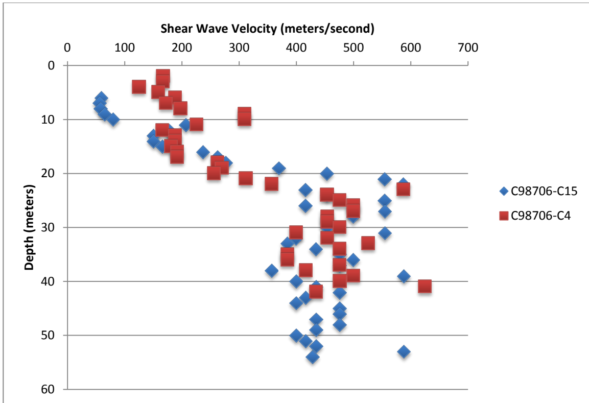
Figure 2. Example shallow shear wave velocity profiles derived from seismic cone penetrometer tests in Charleston. C98706-C15 is located on artificial fill above marsh deposits; C98706-C4 is located on an ~100,000 year old near shore deposit (Wando Formation).
