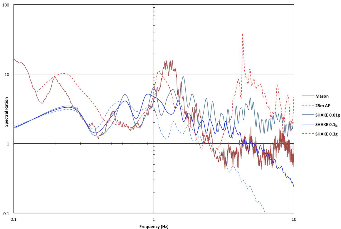
Figure 4. Weak and strong motion response models using SHAKE (blue) versus observed weak motion observation and elastic model for an artificial fill site (red).
