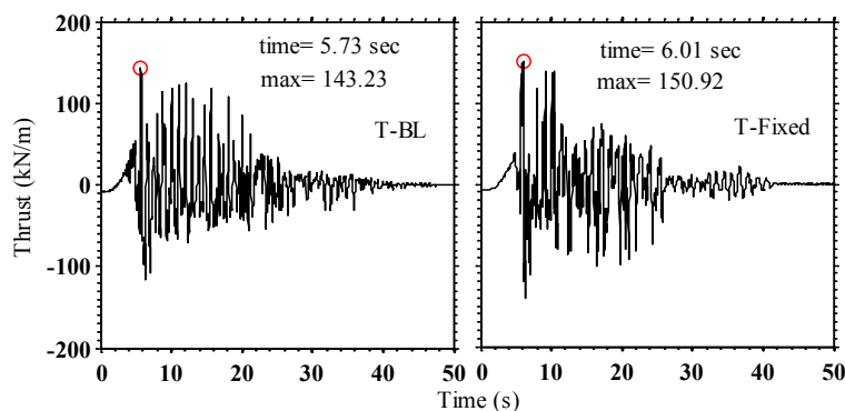
Figure 5. Dynamic thrust time histories during the Northridge-L motion in T-BL and T-Fixed.
