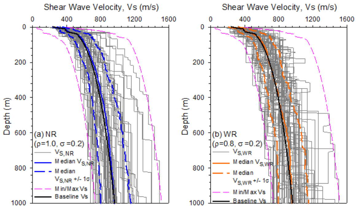
Figure 1. Sixty (60) spatially variable V_S profiles together with the baseline, minimum, and maximum V_S profiles: (a) without V_S reversals, V_{S,NR} ( \sigma_{lnV_S} = 0.2 , \rho_{IL} = 1.0 ) (b) with V_S reversals, V_{S,WR} ( \sigma_{lnV_S} = 0.2 , \rho_{IL} = 0.8 )
