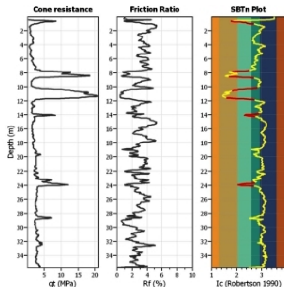
Figure 2. Typical CPT, California Site.
