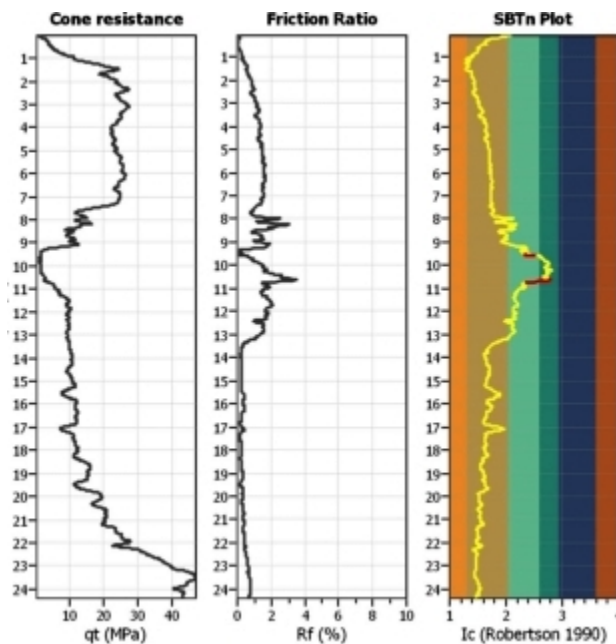
Figure 1. Typical CPT, Western Australia Site
