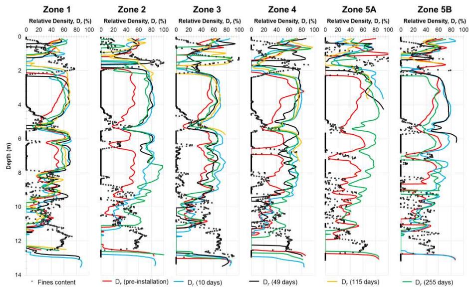
Figure 7. Baseline and time-elapsed post-improvement relative density and fines content as correlated from cone tip resistance
