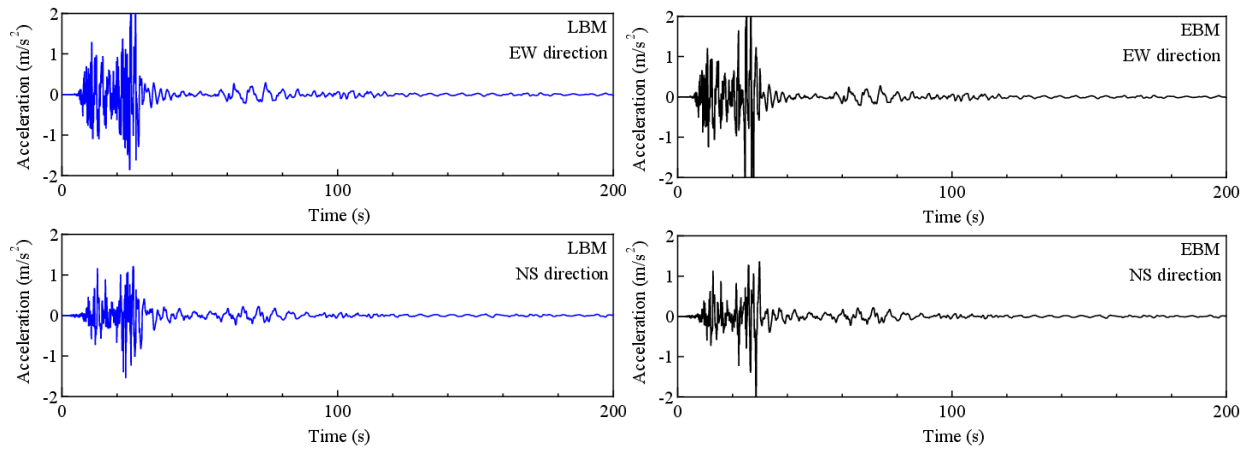
Figure 7: Horizontal acceleration responses at ground surface.
