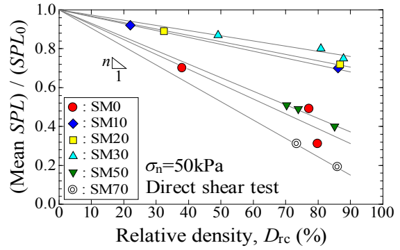
Figure 11. Normalized mean SPL versus Relative density after consolidation.
