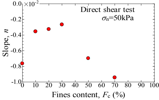
Figure 12. Relation between relative density dependence factor n and fines content.
