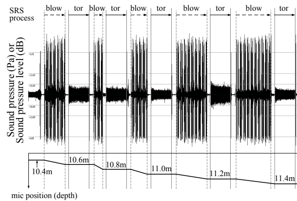
Figure 4. Example of waveform recorded in SRS (Yamada and Oshima, 2015).
