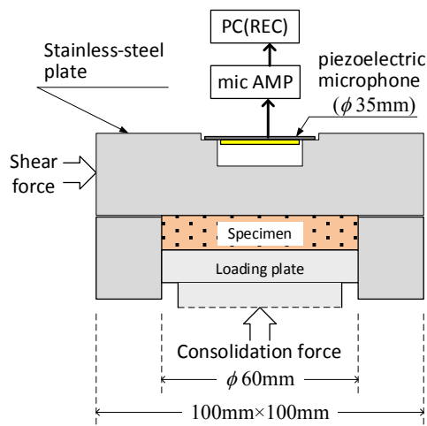
Figure 1. Shear box used for direct box shear test.
