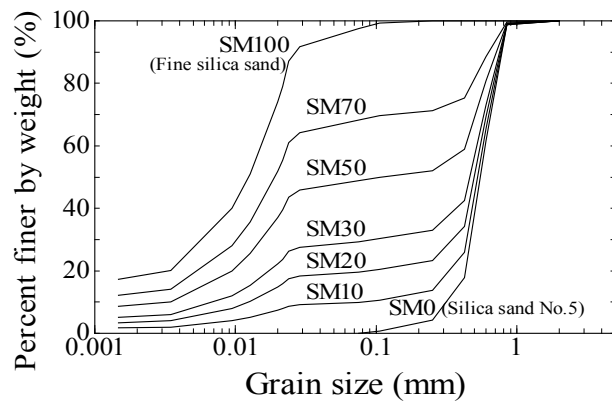
Figure 2. Grain size distribution curves of silica sand mixture used in direct box shear tests.
