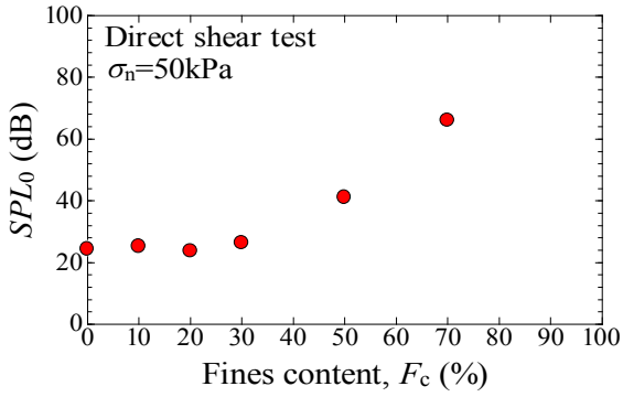
Figure 10. Relationship between SPL for D_{rc}=0\% and fines content
