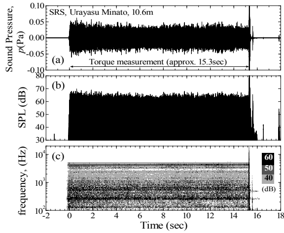
Figure 5. Time histories: (a) sound pressure, (b) sound pressure level and (c) power spectrum.
