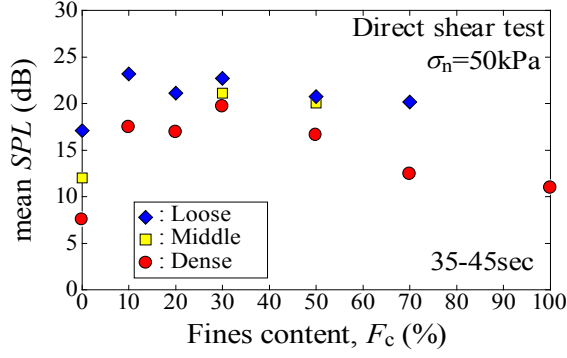
Figure 8. Relation between mean SPL and fines content.
