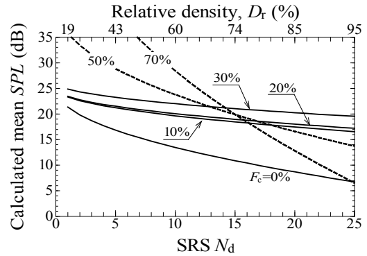
Figure 13. Relation between Calculated mean SPL and SRS N_d -value.
