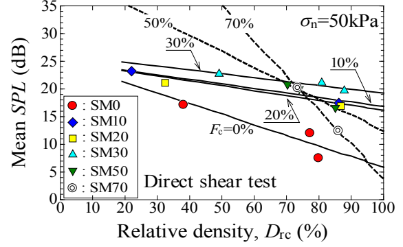
Figure 9. Relation between mean SPL and relative density after consolidation
