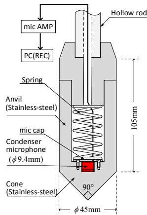
Figure 3. Schematic of penetration cone used for SRS.
