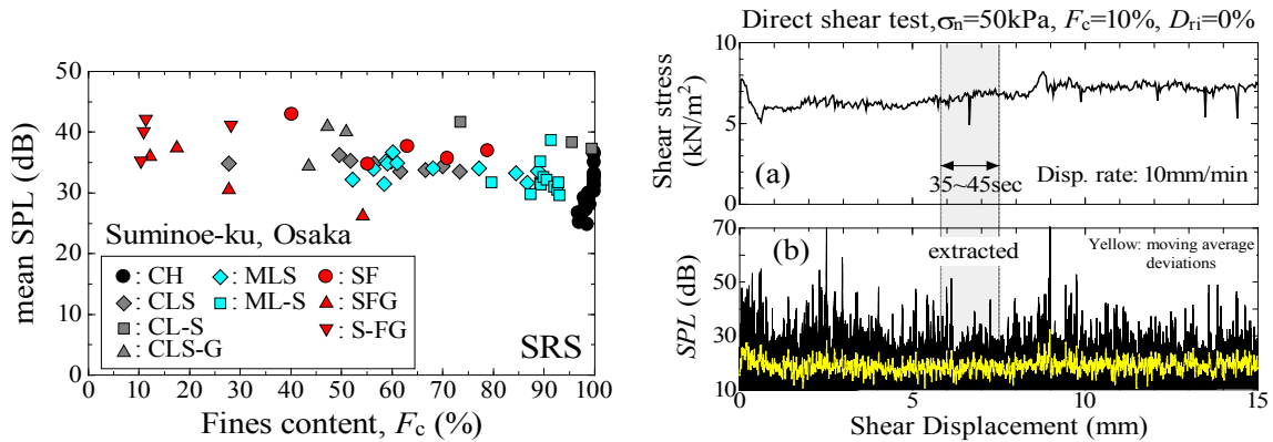
Figure 6. Relation between SPL and fines content, result of field measurement by SRS.
