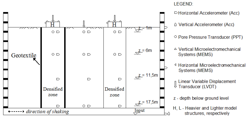
Figure 2. Centrifuge model layout in experiment CT-B (cross section view).
