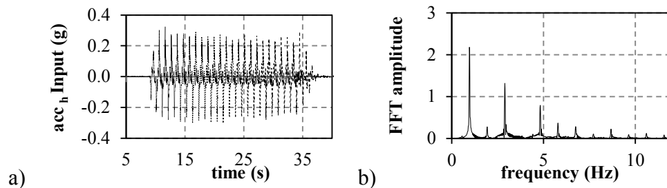
Figure 4. Time history (a) and FFTs (b) of the horizontal seismic motion applied to the model.
