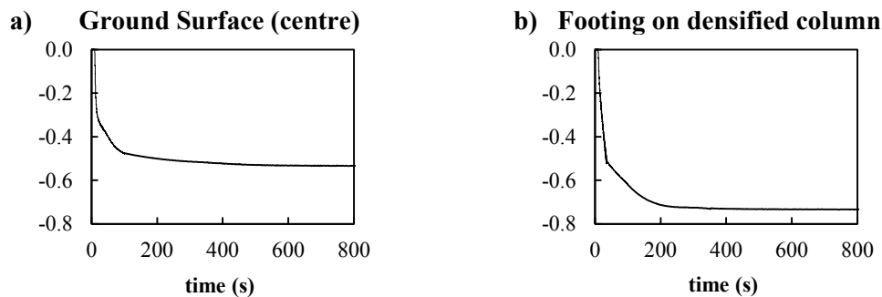
Figure 6. Ground surface (a) and footing (b) settlements (in m)
