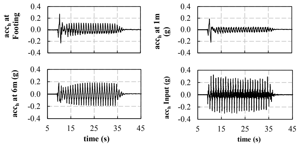
Figure 7. Horizontal accelerations measured at the footing located on top of the narrow densified zone and in the ground under the centre of the same footing at different depths
