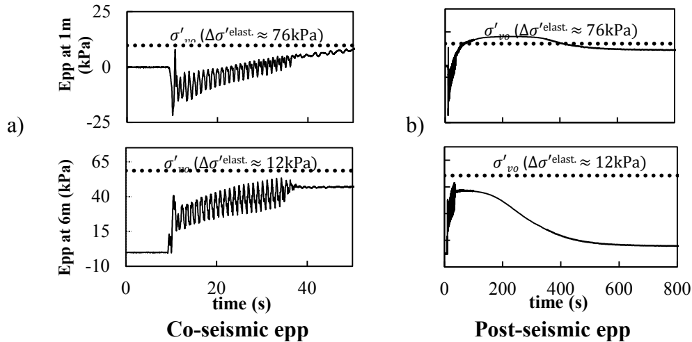
Figure 5. Co- (a) and post- seismic (b) epp at different depths under the footing.
