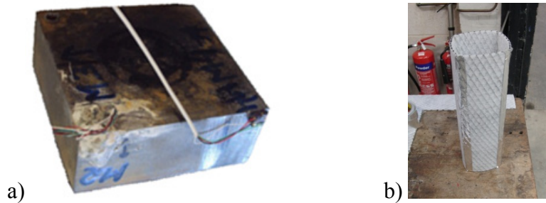
Figure 3. Model structures (a) and geotextile (b) used to simulate high-capacity vertical drains.
