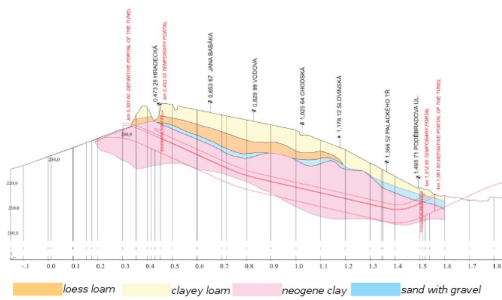
Figure 2. Longitudinal geological cross-section along the tunnels (Pavlik et al. 2004).
