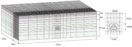
Figure 5. Finite element mesh used in the analyses of the exploratory drift.
