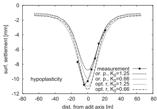
Figure 6. Surface settlement troughs due to exploratory drift predicted with the original parameter set (“or. p.”) and with optimized value of the parameter r (“opt. r ”).
