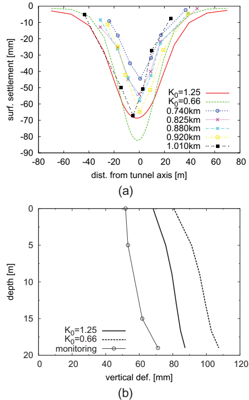
Figure 9. Surface settlement trough (a) and extensometer measurements (b). Class A predictions compared with the monitoring data.
