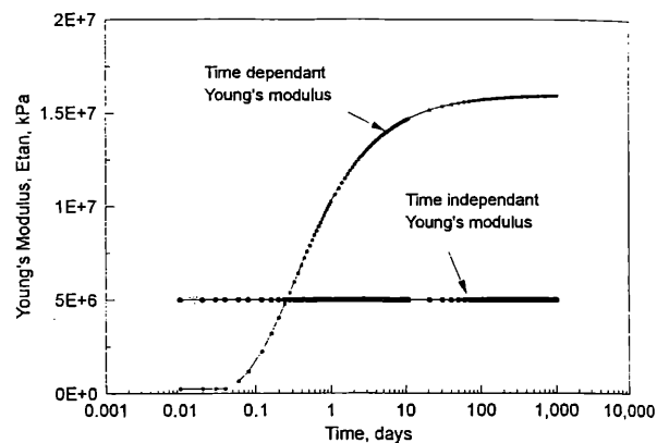
Fig. 2 Assumed Young's modulus-time relation for shotcrete
