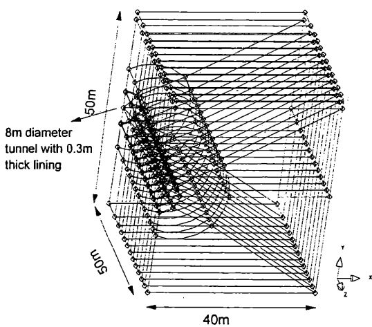
Fig. 4 Geometry for 3D analysis
