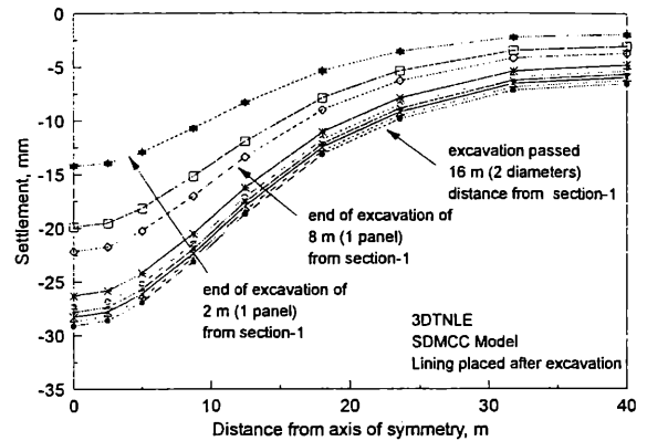
Fig. 8 The surface settlement profiles at the cross section-1
