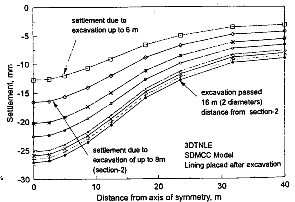
Fig. 9 The surface settlement profiles at Section-2
