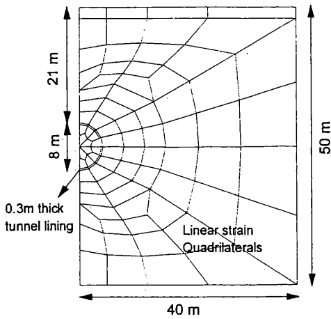
Fig. 3 Mesh adopted for 2D analysis
