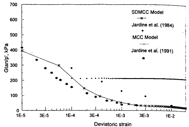
Fig. 1 Shear stiffness-strain variation for London Clay
