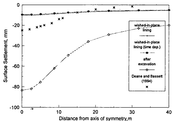
Fig. 6 Effect of construction sequence on surface settlements
