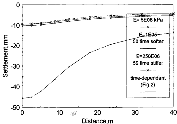
Fig. 7 Effect of shotcrete stiffness on settlement profiles
