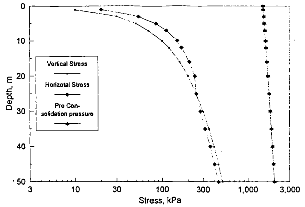
Fig. 5 In-situ effective stress state for London Clay
