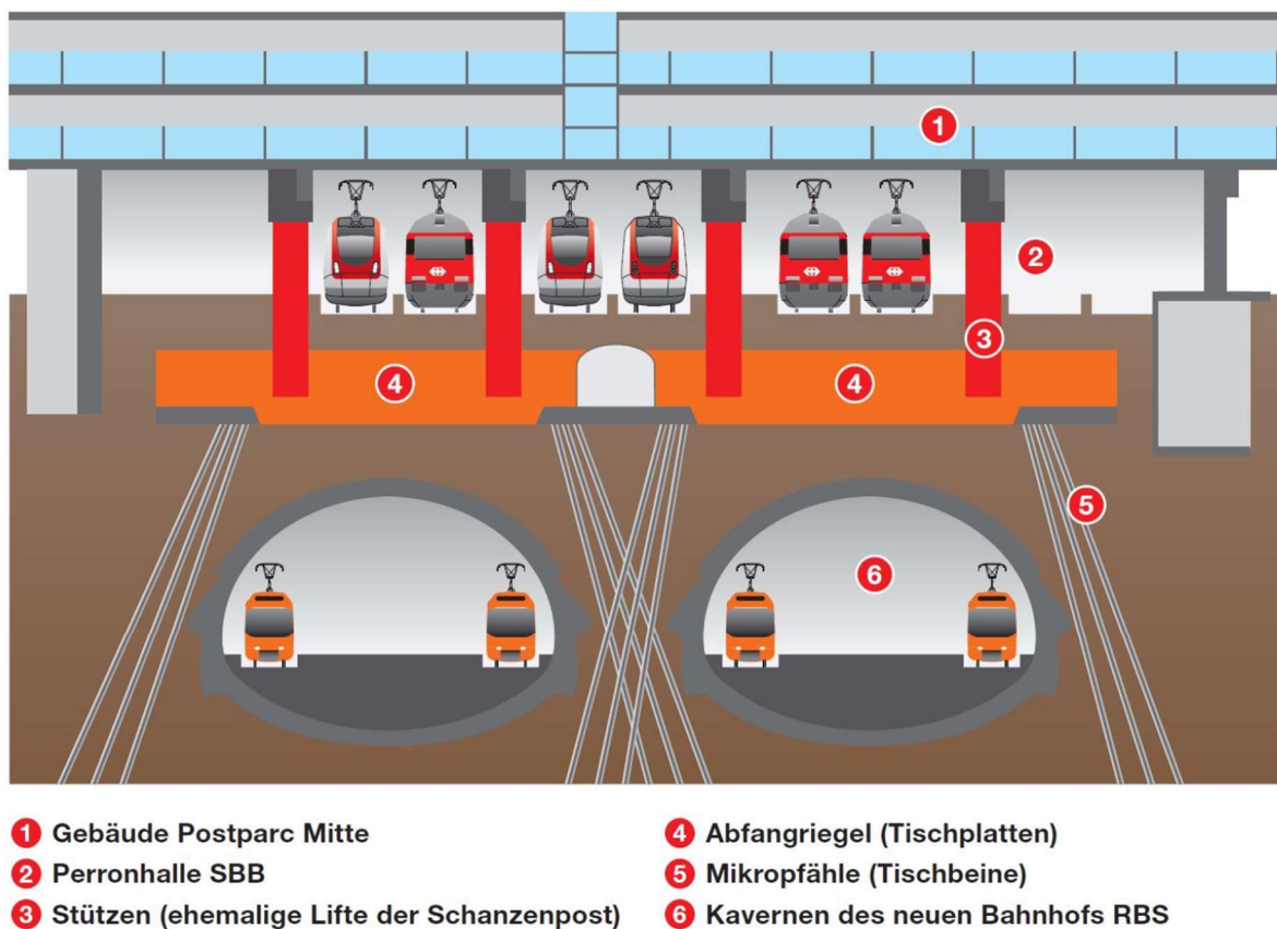
Figure 4: Designed situation with the new foundation of the Postparc building and the new caverns (source: https://www.zukunftbahnhofbern.ch )
