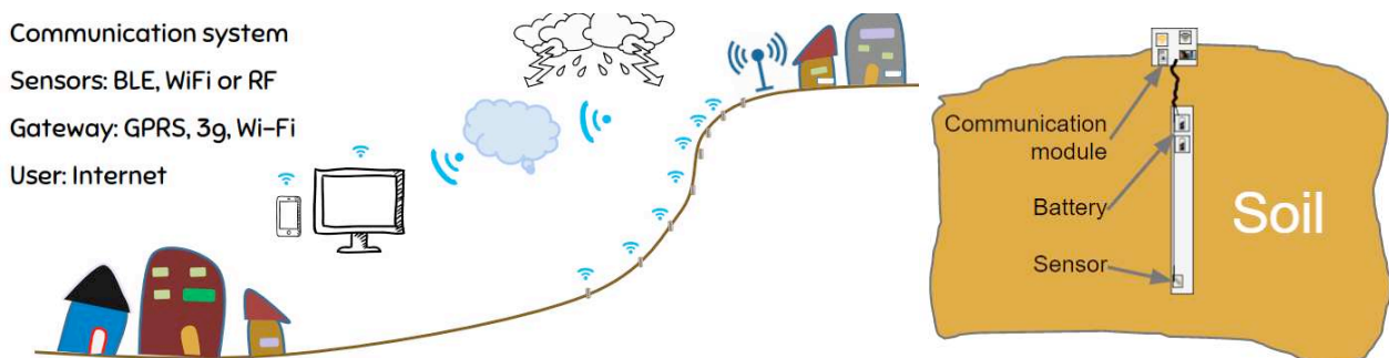
Figure 4. Monitoring system with vibration sensor.
