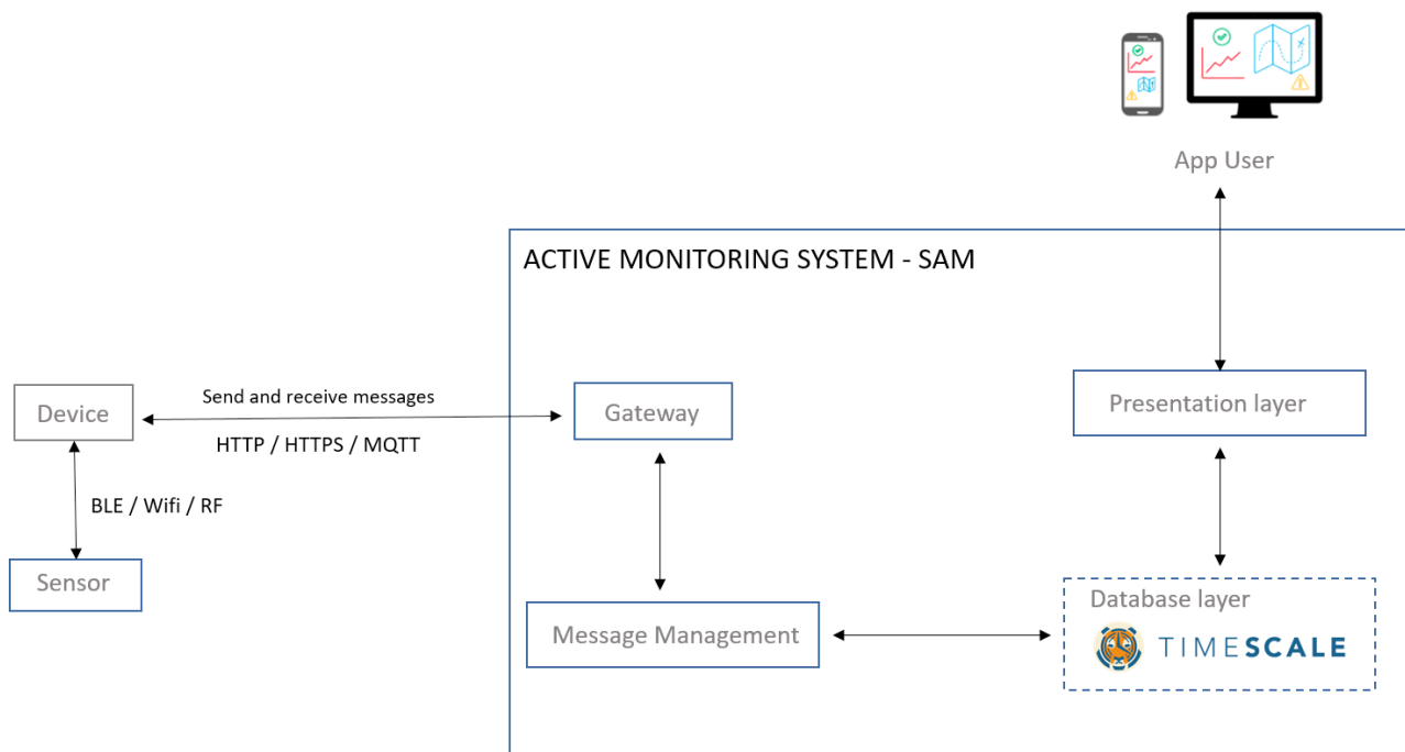
Figure 2. Cloud architecture
