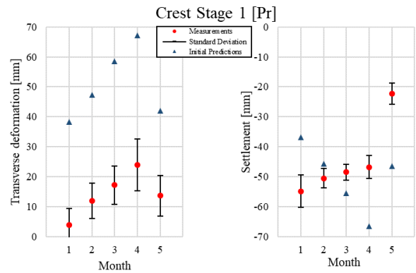
Figure 5. Comparison in the prisms: (a) Transverse deformations and (b) Settlements, between measurements and initial predictions
