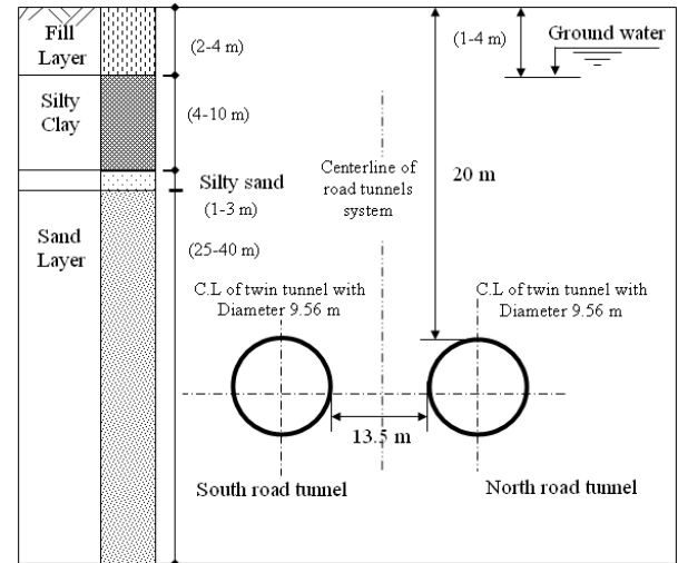
Fig. 2: Soil profile along El-Azhar road tunnels
