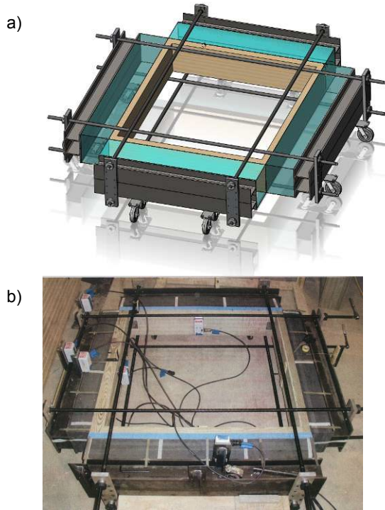
Figure 7. Test apparatus designed to simulate expansive soil loading a) CAD model, b) Physical test apparatus
