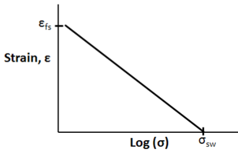
Figure 1. Vertical strain versus overburden stress
