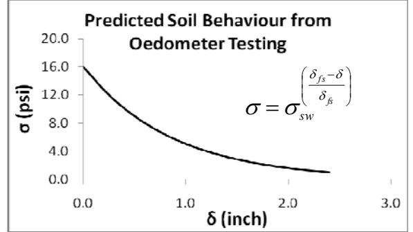
Figure 3. Ideal soil behavior using \sigma_{sw}=16 psi and \delta_{fs}=2.4 inches
