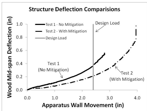
Figure 9. Test comparisons between mitigated and non-mitigation structure designs
