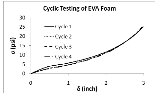
Figure 6. Foam cyclic testing results
