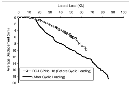
Figure 14. Stage 3 – RG-HSP 18 lateral load-displacement (before and after cyclic loading)
