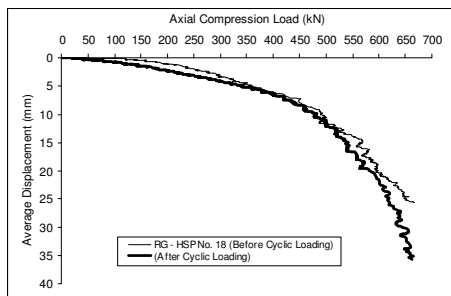
Figure.7. Load-displacement curves for RG-HSP 18 before and after cyclic loading
