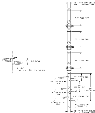
Figure.1. Schematic of an SS 175 AB Chance Helical Screw Foundation System.
