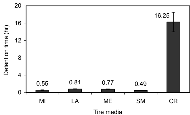
Figure 8. Detention time affected by different tire materials.
