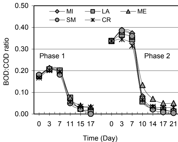
Figure 3. The BOD:COD ratio of different tire materials.
