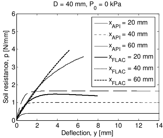
Figure 12. p - y curves for three depths from the numerical model and the design regulation formulation for the 40 mm pile with P_0 = 0 kPa.
