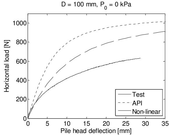
Figure 13. Load-deflection relationships measured at the height of the hydraulic piston ( x = -370 mm) obtained from the tests and the Winkler model approach with the expressions for the ultimate soil resistance with both linear and non-linear formulation of the initial stiffness incorporated. D = 100 mm. P_0 = 0 kPa. The initial modulus of subgrade reaction, k , is set to 40000 \text{ kN/m}^3 .
