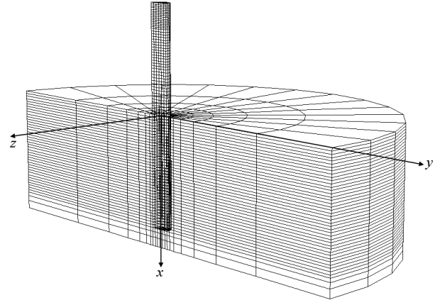
Figure 2. Zone geometry in the models with 100 mm pile.
