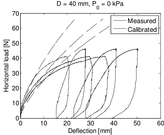
Figure 5. Calibrated and measured relationships at three levels above the soil surface for the test 40 mm with P_0 = 0 kPa.
