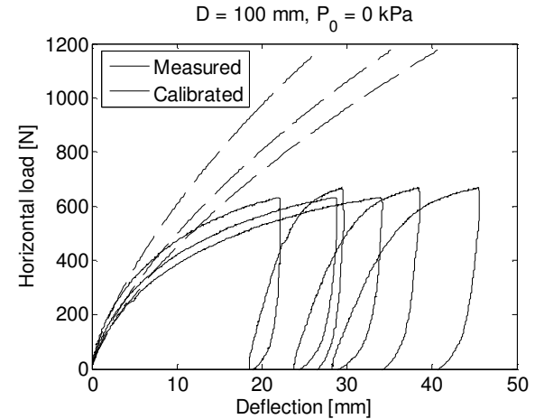
Figure 3. Calibrated and measured relationships at three levels above the soil surface for the test 100 mm with P_0 = 0 kPa.
