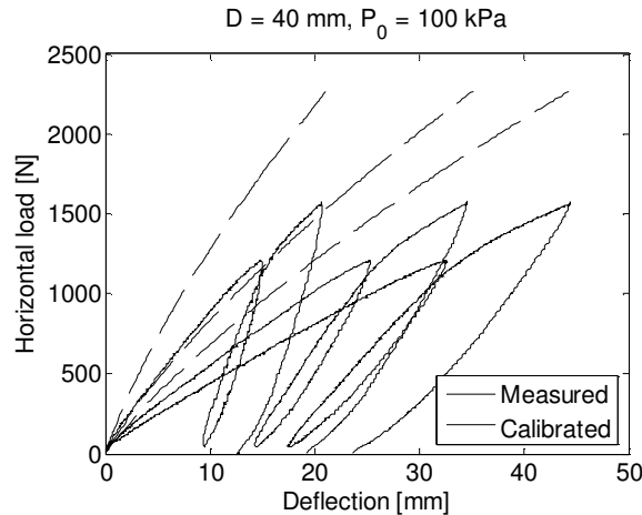
Figure 6. Calibrated and measured relationships at three levels above the soil surface for the test 40 mm with P_0 = 100 kPa.
