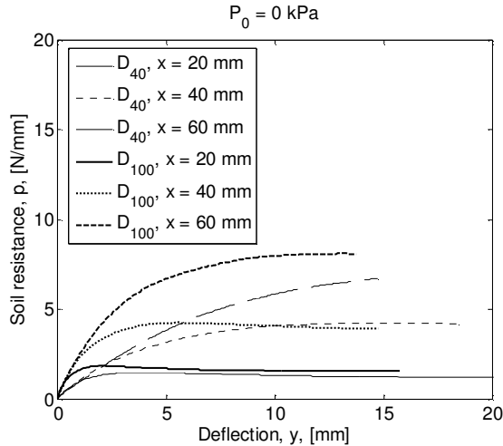
Figure 8. p - y curves at three different depths for models with 40 mm and 100 mm piles and P_0 = 0 kPa.
