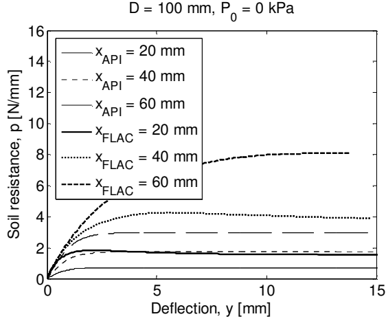
Figure 11. p - y curves for three depths from the numerical model and the design regulation formulation for the 100 mm pile with P_0 = 0 kPa.
