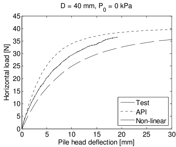
Figure 14. Load-deflection relationships measured at the height of the hydraulic piston ( x = -370 mm) obtained from the tests and the Winkler model approach with the expressions for the ultimate soil resistance with both linear and non-linear formulation of the initial stiffness incorporated. D = 40 mm. P_0 = 0 kPa. The initial modulus of subgrade reaction, k , is set to 40000 \text{ kN/m}^3 .
