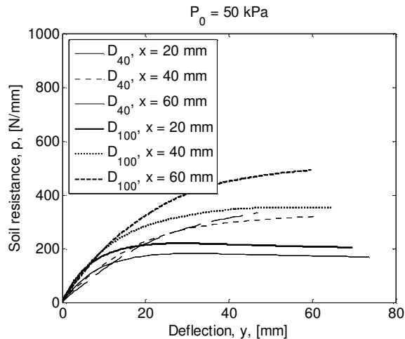
Figure 9. p - y curves at three different depths for models with 40 mm and 100 mm piles and P_0 = 50 kPa.
