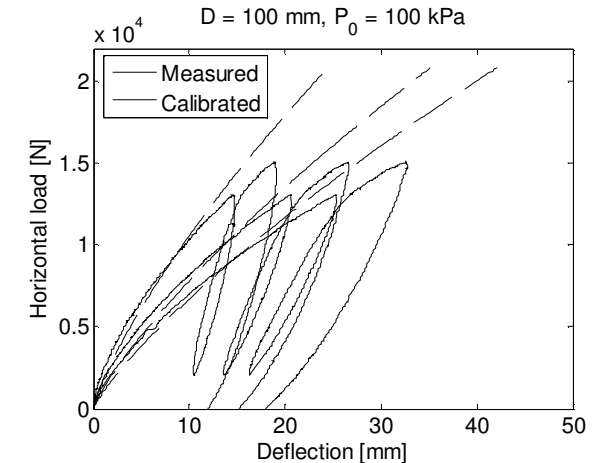
Figure 4. Calibrated and measured relationships at three levels above the soil surface for the test 100 mm with P_0 = 100 kPa.
