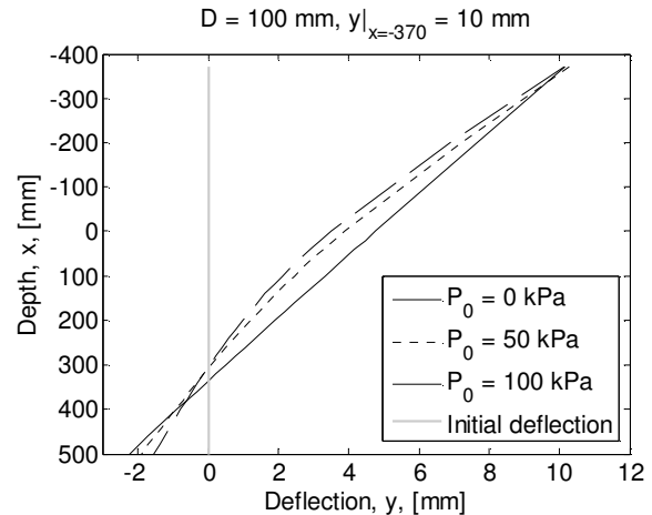
Figure 7. Lateral deflection with depth for different overburden pressures for the 100 mm piles.
