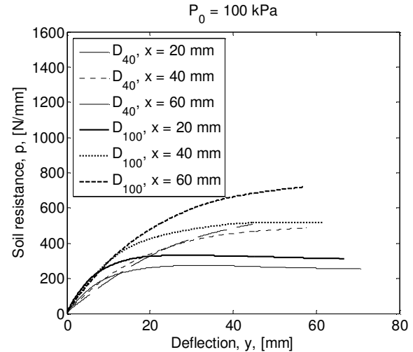
Figure 10. p - y curves at three different depths for models with 40 mm and 100 mm piles and P_0 = 100 kPa.
