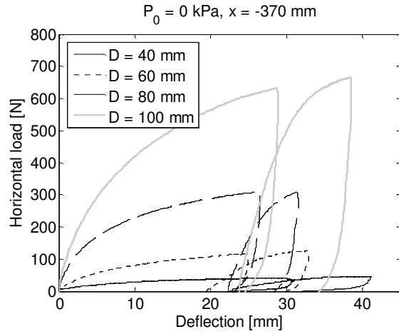
Figure 14. Load-deflection relationships for the four piles at P_0 = 0 kPa.
