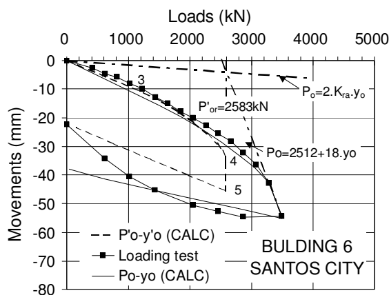
Figure 10. Loads-movements
