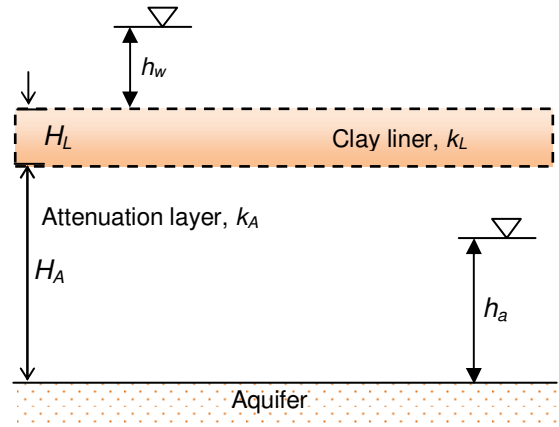
Figure 3 Clay liner over an attenuation layer and aquifer
