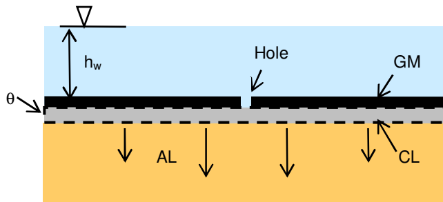
Figure 7 Schematic showing leakage, Q , through a hole in a GM over a CL
