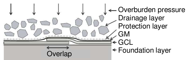
Figure 11 Schematic of a GCL panel overlap (adapted from Brachman et al. 2011)
