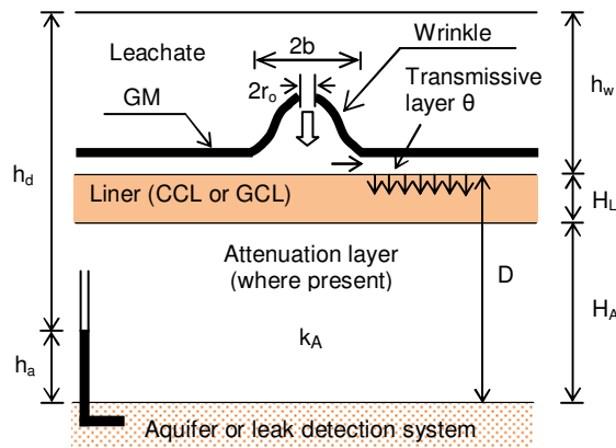
Figure 8 Schematic showing leakage through a wrinkle of length L and width 2b with a hole of radius r_o (adapted from Rowe 1998)
