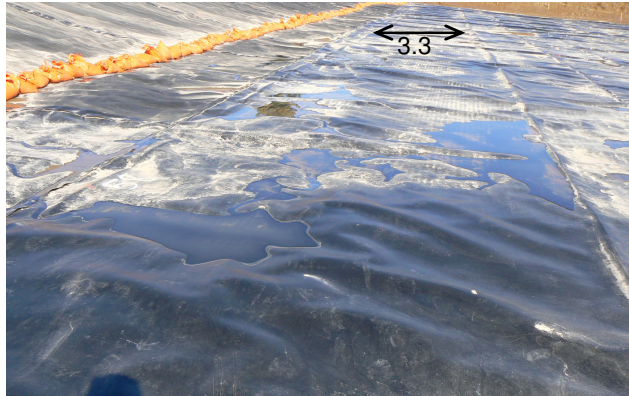
Figure 9 Photograph of wrinkles at QUELTS (same bottom liner as shown in Figure 6) on 23 March 2007 when ambient temperature is 9°C. Note longitudinal wrinkles at 3.3 m spacing are beginning to form. White patches are what remain of a sprinkling of snow on liner from the previous night. Water puddles from melting snow are constrained from flowing off the base (slope 3% from left to right—north to south) by the wrinkles.
