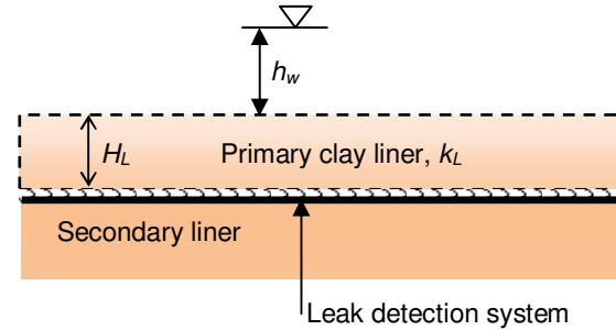
Figure 2 Clay liner over a leak detection system
