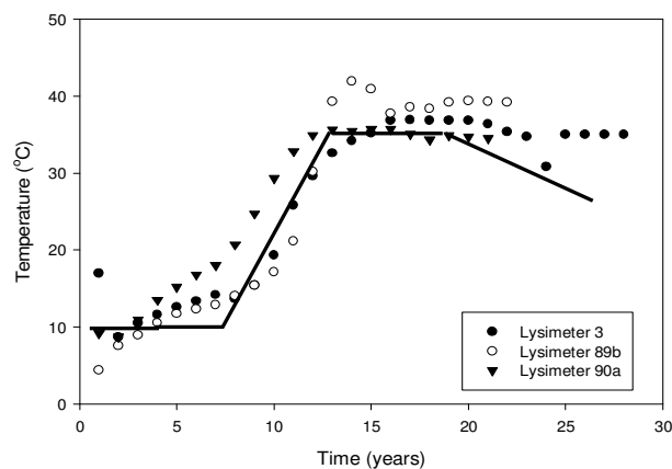
Figure 12 Most recent available data for liner temperatures at three locations at the Keele Valley Landfill, Toronto and an idealized temperature time history (Data courtesy of the City of Toronto and Golder Associates)
