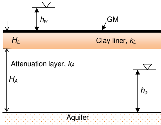
Figure 5 Single composite liner over an attenuation layer and aquifer (also depicts secondary composite liner in a double lined system)
