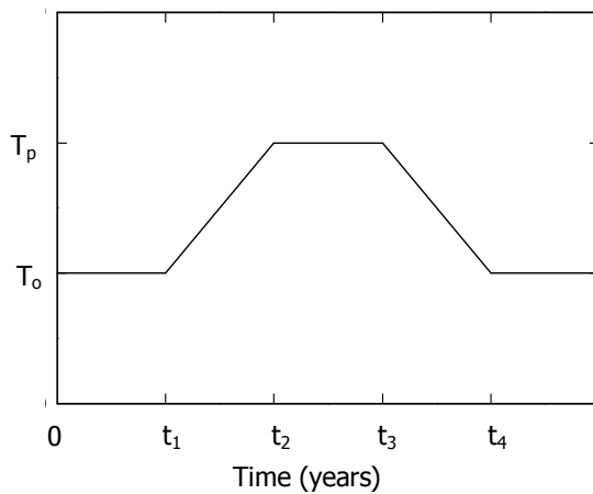
Figure 13 Schematic of a temperature-time history for a landfill liner; T_o is initial and final temperature; T_p is peak liner temperature (modified from Rowe and Islam 2009)
