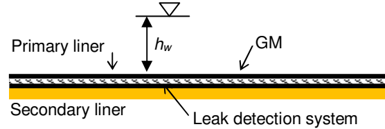
Figure 1 Single GM primary liner over a leak detection system
