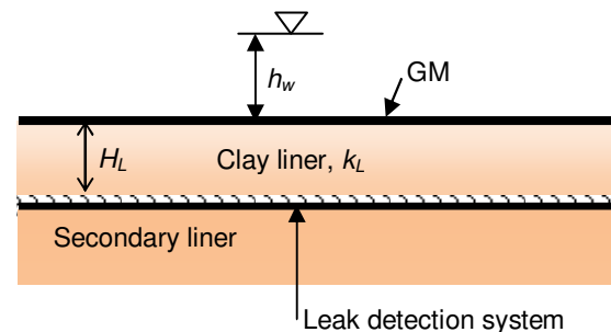
Figure 4 Primary composite liner over a leak detection system
