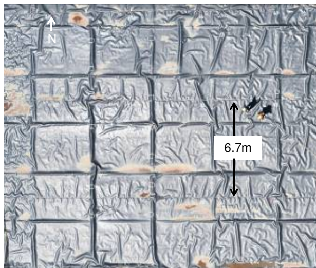
Figure 10 Aerial photo showing a small portion of connected wrinkle network on the base liner at QUELTS (same bottom liner as shown in Figures 6 and 9) Taken on 28 May 2008 at 1:00 pm; air temperature of 11°C; GM temperature on the base of 53°C. Distance between GM seams is approximately 6.7 m as shown. Modified from Rowe et al. (2011b).
