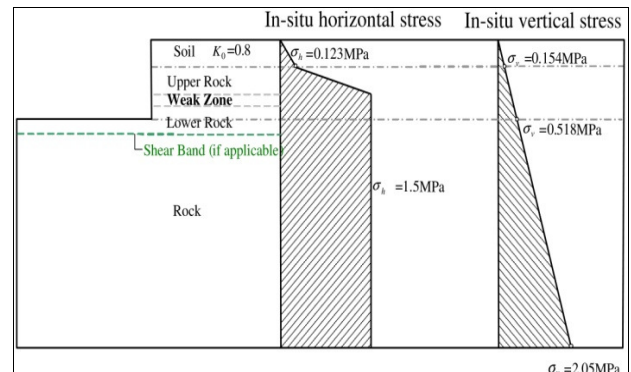
Figure 21. Assumed vertical and lateral in-situ stresses
