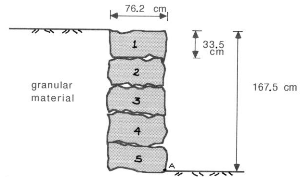
Figure 3. Dimensions of the Inca wall used for the stability analysis
