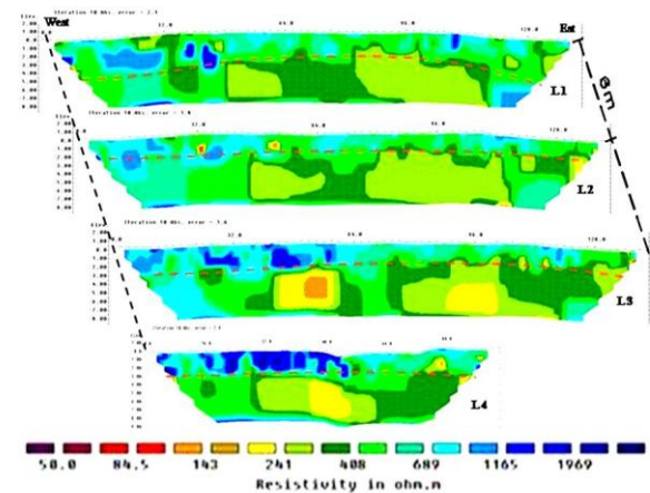
Figure 3. Resistivity models resulting from 2D inversion of ERT lines (L1, L2, L3 and L4) separated by a distance of 6 m.
