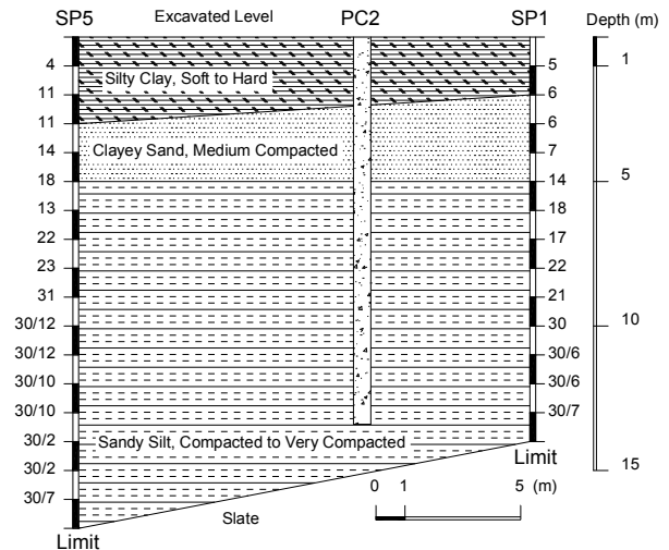
Figure 2. Typical geotechnical profile of the site
