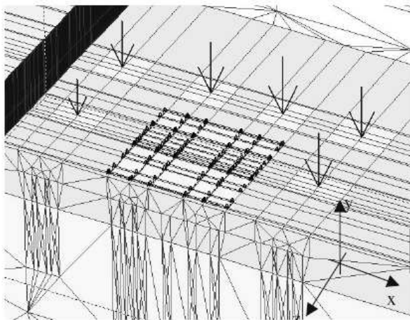
Figure 6. Details of the 3D adopted mesh
