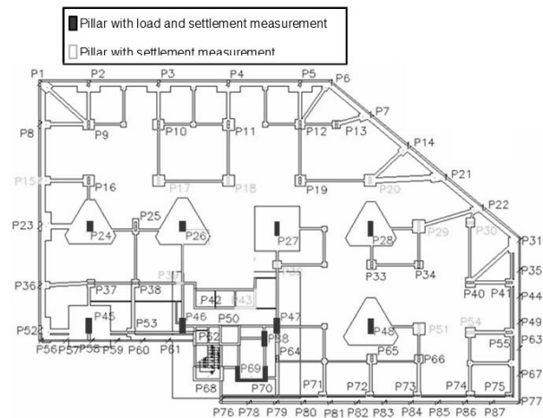
Figure 4. Instrumented columns of the building
