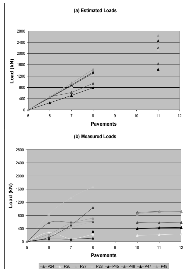
Figure 7. Comparison of column loads
