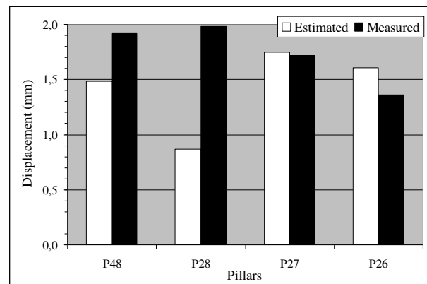
Figure 8. Comparison of underground settlements
