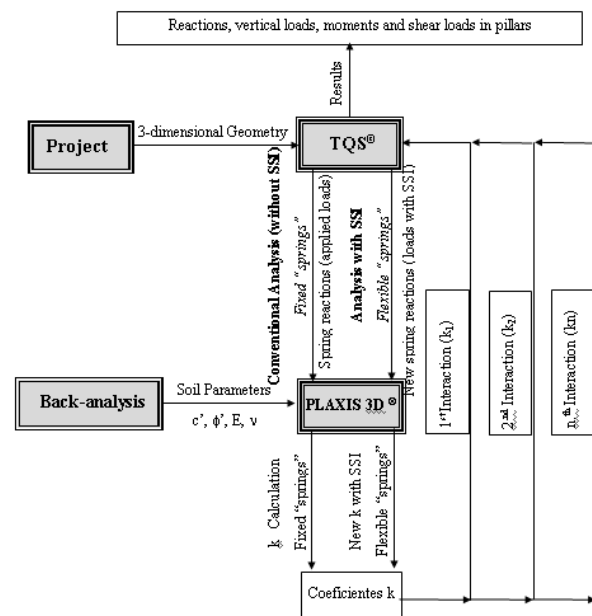
Figure 5. Flowchart for SSI uncoupled analysis
