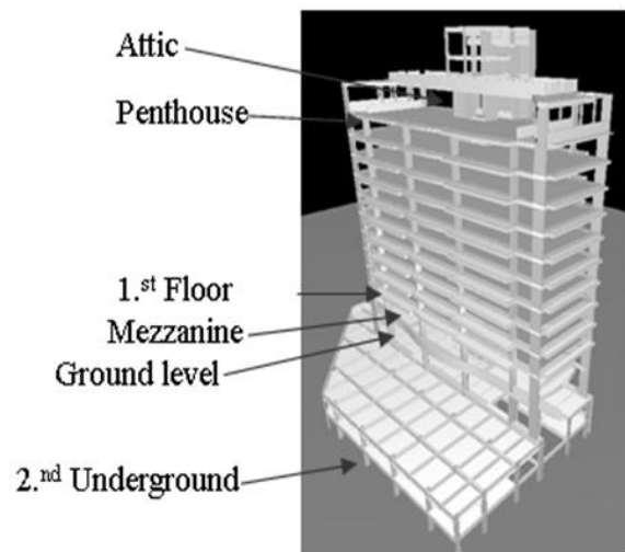
Figure 3. General view and aspects of the building
