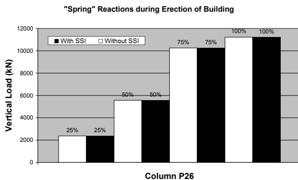
Figure 10. Vertical load of column 26 at distinct stages
