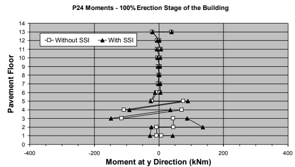
Figure 11. M_y values of column 24 at distinct levels
