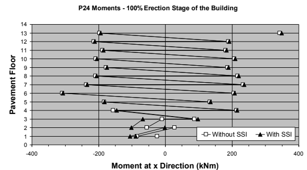
Figure 12. M_x values of column 24 at distinct levels
