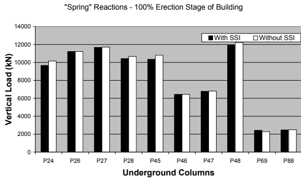
Figure 9. Vertical column loads with and without SSI
