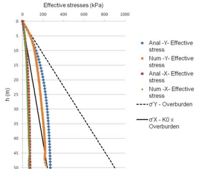
Figure 3: Vertical and horizontal effective stresses profiles along the VCL obtained from the numerical simulation and the analytical solution (Case 1).
