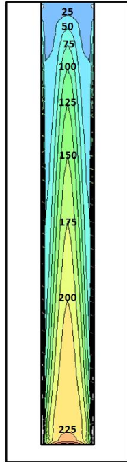
Figure 4 : Iso-contours of the vertical stresses within the backfill (Case 1; values given in kPa).
