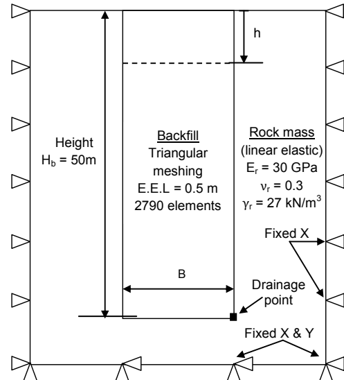
Figure 2: Stope geometry and finite element mesh
