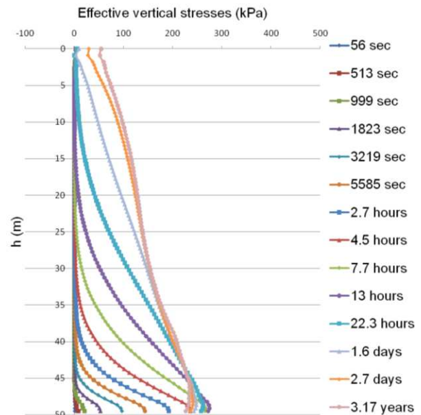
Figure 9: Evolution of the effective vertical stress \sigma'_v along the VCL within the backfilled stope (Case 3)
