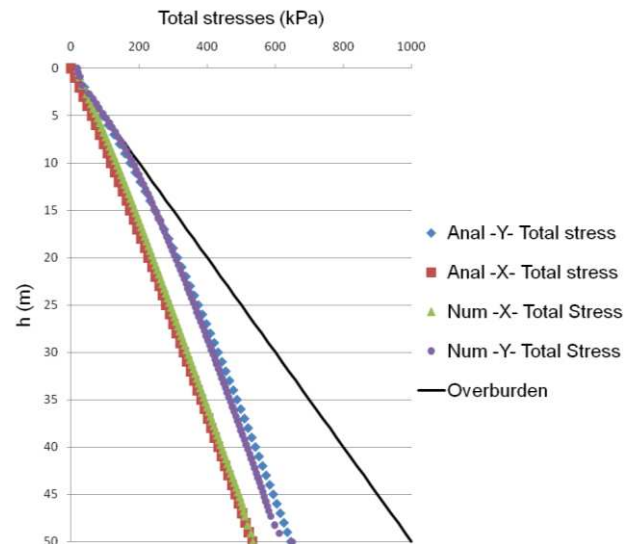
Figure 6: Vertical and horizontal total stresses within the backfilled stope, obtained from the numerical simulation and analytical solution (Case 2)
