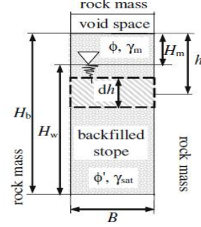
Figure 1: A vertical stope with partially submerged backfill (adapted from Li and Aubertin, 2009a)
