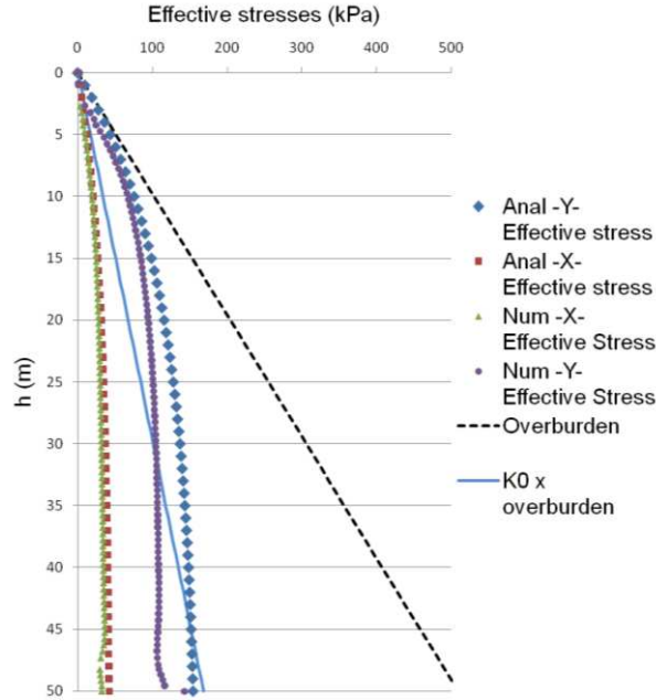
Figure 7: Effective stresses (horizontal and vertical) profiles obtained from the numerical calculation and analytical solution (Case 2)
