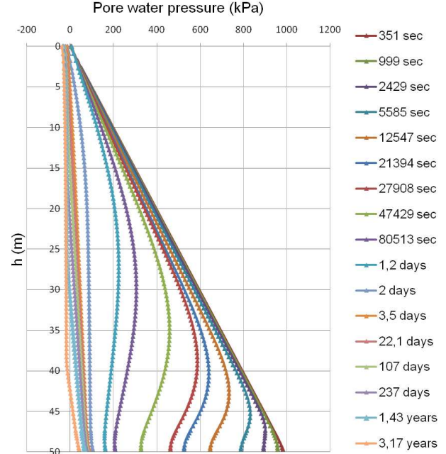
Figure 8: Evolution of the pore water pressure along the VCL of the initially saturated backfilled stope (Case 3)
