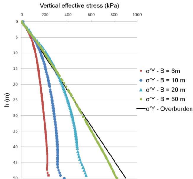
Figure 5: The effect of slope width B on the vertical stress along the VCL (Case 1).
