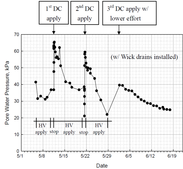
Figure 8. Pore pressure response due to PVDs and vacuum dewatering.
