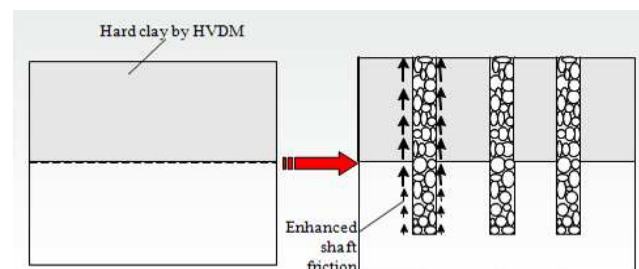
Figure 3. HVDM plus stone columns as composite foundation.
