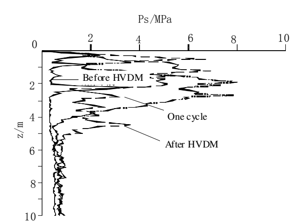
Figure 6. Comparison of CPT cone resistance between before and after HVDM.
