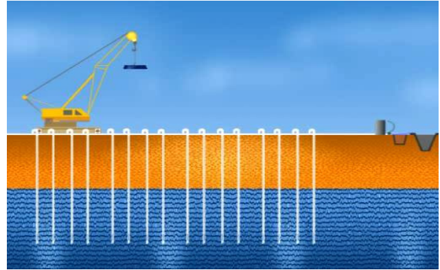
Figure 1. Schematics of HVDM method.
