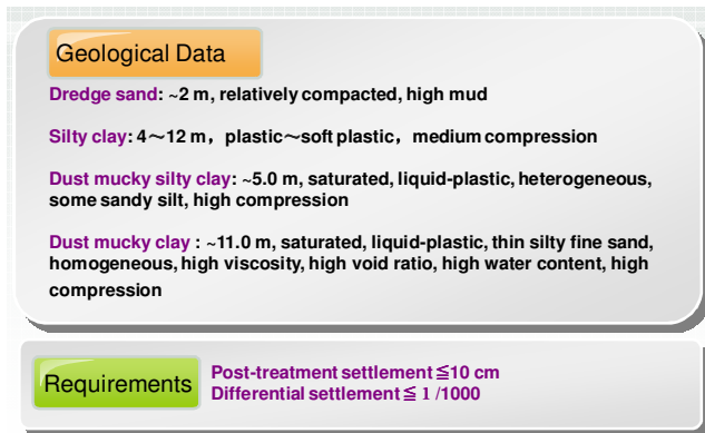
Figure 4. Soil profile at Shanghai Pudong Airport Runway No. 2 Project.
