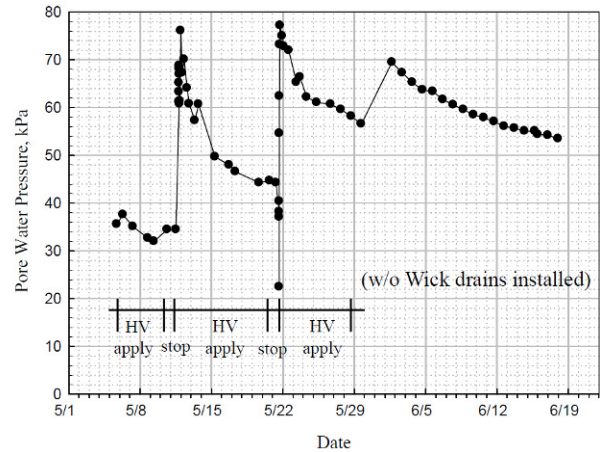
Figure 9. Pore pressure response due to PVDs and variation.
