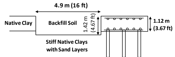
Figure 1. Profile view of the South Temple [5.18 m (17 ft) wide cap] test configuration.
