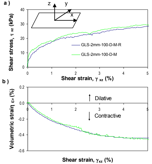
Figure 2. Results of DSS tests GLS-2mm-100-D-M and GLS-2mm-100-D-M-R a) Shear stress strain response b) volumetric strain vs. shear strain.
