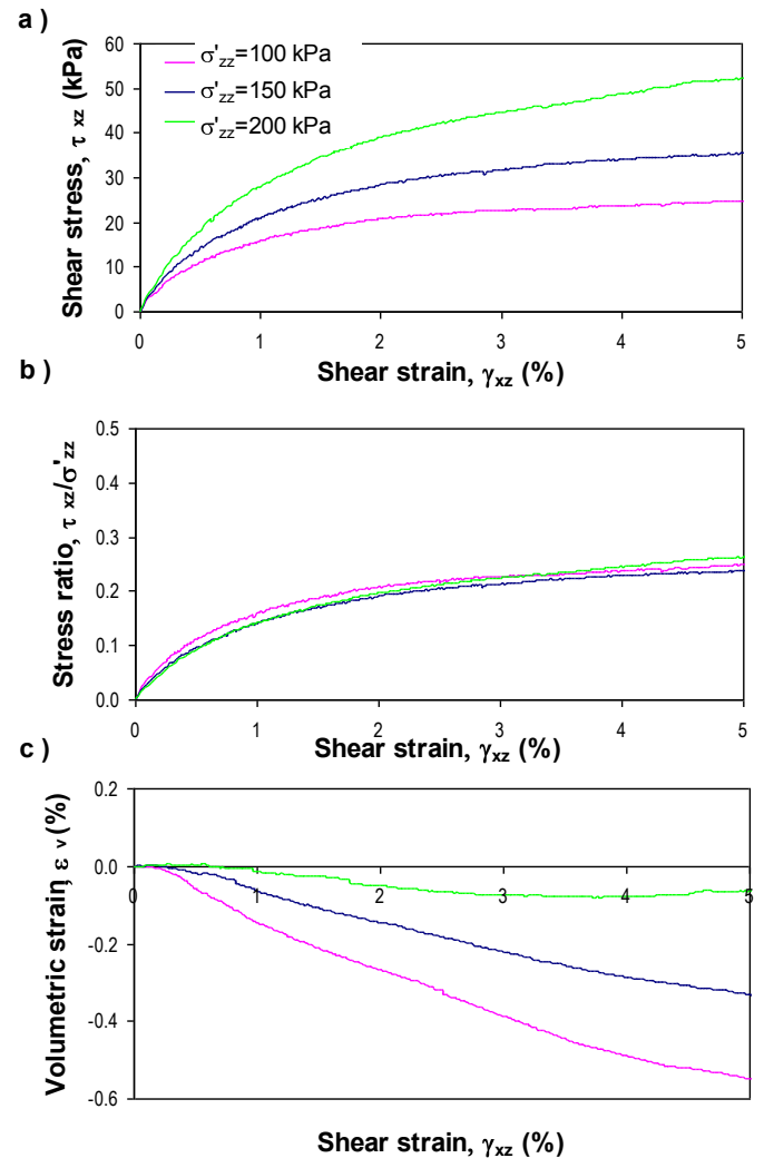
Figure 6. Shear response from DSS-PFC 3D model for K = 50 kN/m and F=0.2 for \sigma'_{zz} values of 100 kPa, 150 kPa, and 200 kPa: a) Shear stress strain response; b) Stress ratio shear strain response; and c) volumetric strain vs. shear strain.
