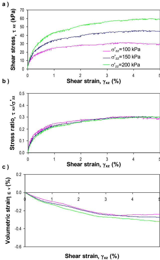
Figure 5. Shear response from DSS-PFC 3D model for K = 500 kN/m and F = 0.2 for \sigma'_{zz} values of 100kPa, 150kPa, and 200kPa: a) Shear stress strain response; b) Stress ratio shear strain response; c) volumetric strain vs. shear strain.
