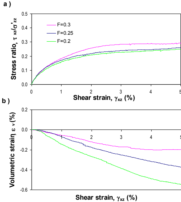
Figure 7. Shear response from DSS-PFC 3D model for K = 50 kN/m and F values of 0.2, 0.25, and 0.3: a) Stress ratio shear strain response; and b) volumetric strain versus shear strain.
