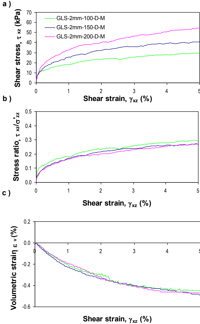
Figure 3. Results of DSS tests GLS-2mm-100-D-M, GLS-2mm-150-D-M, and GLS-2mm-200-D-M a) Shear stress strain response b) Stress ratio shear strain response c) volumetric strain vs. shear strain.
