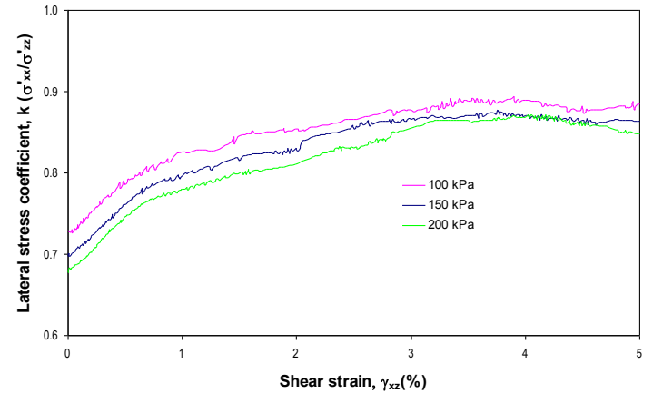
Figure 8. Variation in coefficient of lateral stress with the development of shear strain for DSS tests simulated with \sigma'_{zz} values of 100 kPa, 150 kPa, and 200 kPa (for K = 500 kN/m and F = 0.2 ).
