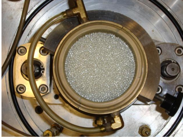
Figure 1. 2mm air pluviated glass beads in the DSS cylindrical cavity at the end of specimen preparation.
