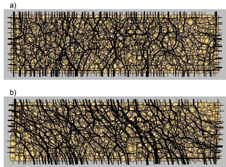
Figure 9. A central cross section through the simulated DSS specimen parallel to the x-axis showing contact forces: a) at the end of consolidation and prior to shearing; and b) at 4% shear strain.
