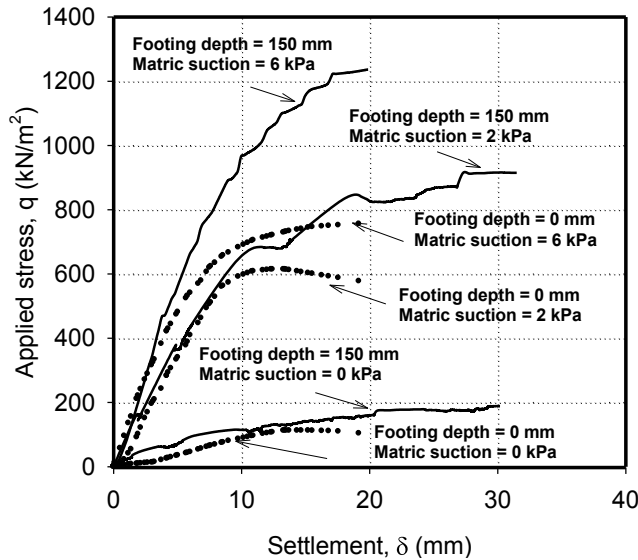
Figure 2. Relationship between the applied stress versus settlement behaviour of surface and embedded model footing tests (PLTs) of 150 mm × 150 mm
