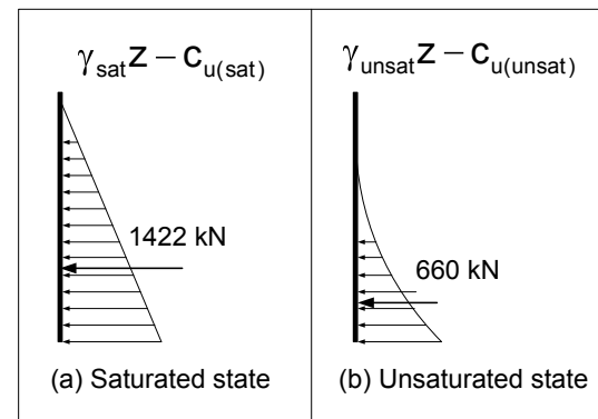
Fig. 13. Earth pressure distribution extending effective stress approach (a) conventional approach and (b) proposed approach using the mechanics of unsaturated soils.
