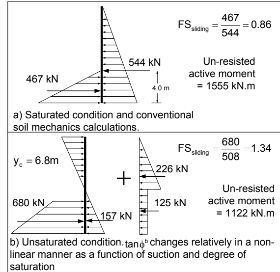
Figure 12. Earth pressure distribution extending effective stress approach (a) conventional approach and (b) proposed approach using the mechanics of unsaturated soils.
