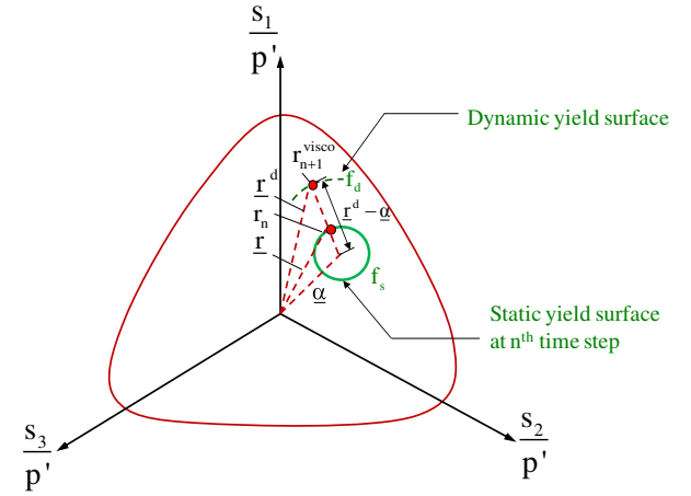
Figure 4. (a) The concept of overstress viscoplastic model (from Liingaard et al. 2004) and (b) initial ('static') and dynamic yield surfaces in the current model
