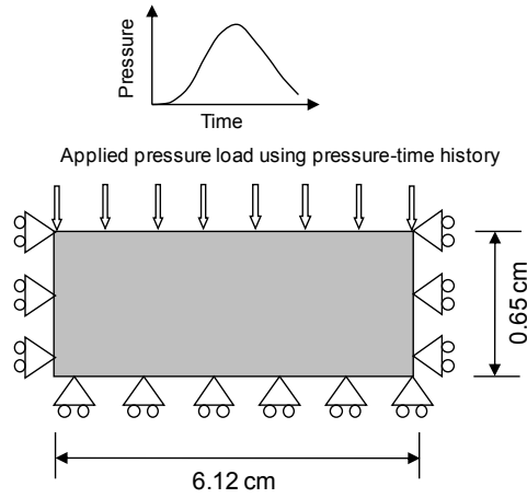
Figure 6. Geometry of the SHPB test sample
