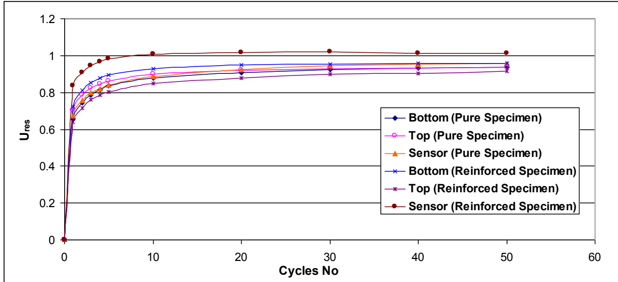
Figure 8. Normalized residual excess pore water pressure change with increase of cycles at top, middle and bottom of specimens having inclusion-free and inclusion-surrounded IPT (vertical) inside
