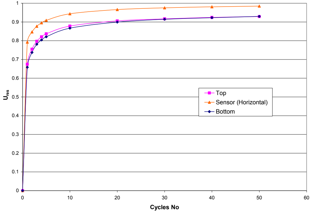
Figure 10. Normalized residual excess pore water pressure change with increase of cycles at top, middle and bottom of specimens having free and inclusion-surrounded IPT (horizontal) inside
