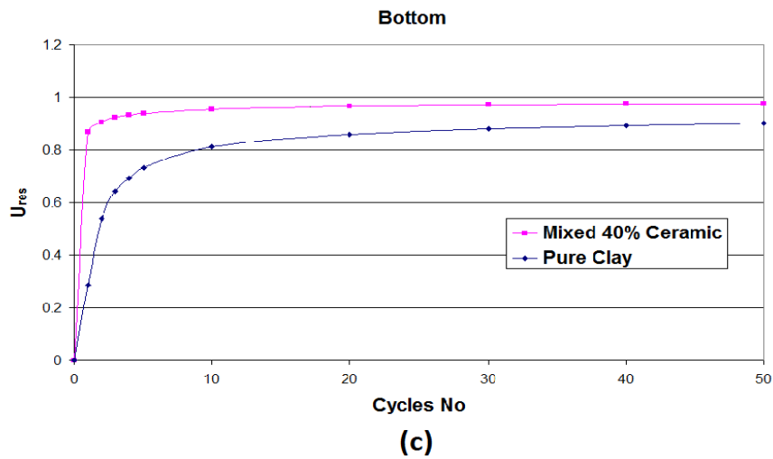
Figure 7. Normalized residual excess pore water pressure change with increase of cycles at frequency of 0. 005 Hz at a) top; b) middle; c) bottom of the specimens ( U = EPWP / \text{Initial Effective Confining Pressure} )
