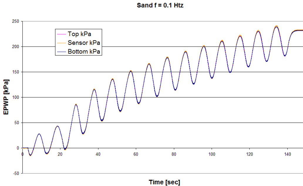
Figure 3. Excess pore water pressure (EPWP) change with time in the test on loose sandy specimen: IPT (mentioned as sensor in the legend) measurement was well in agreement with top and bottom measurements
