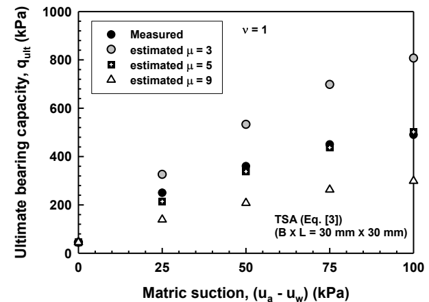
Figure 12. Comparison between the measured and the estimated bearing capacity values extending the TSA ( v = 1 and different \mu values).
