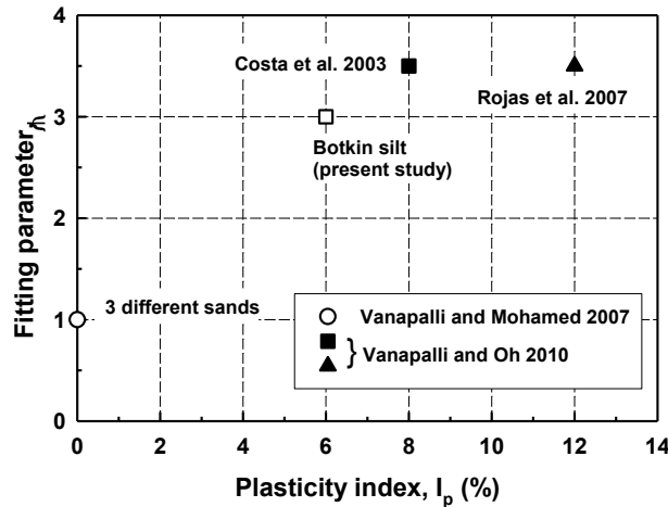
Figure 10. Relationship between fitting parameter, \psi and plasticity index, I_p .
