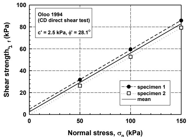
Figure 8. Effective shear strength envelopes for Botkin silt used in the present study.
