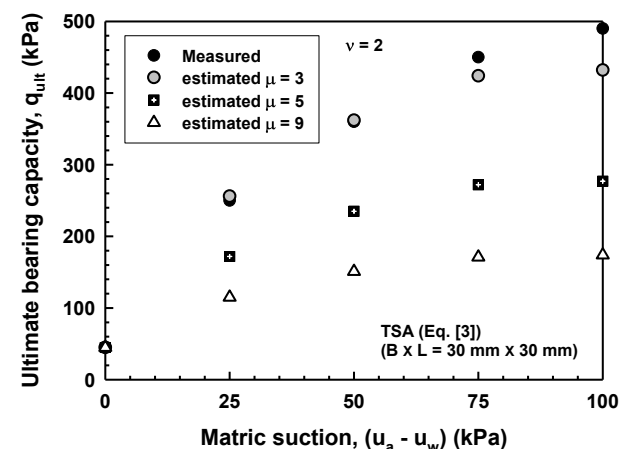
Figure 13. Comparison between measured and estimated bearing capacity values extending the TSA ( v = 2 and different \mu values).
