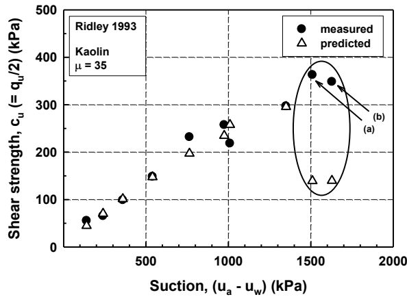
Figure 5. Comparison between the measured and the predicted undrained shear strength (data from Ridley 1993).
