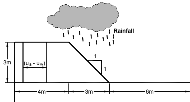
Figure 9. Cross-section of the embankment used in the present study
