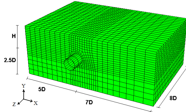
Figure 1: The finite element model geometry
