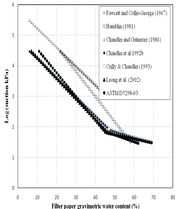
Figure 1. Evaluated calibration curves for Whatman 42 filter paper
