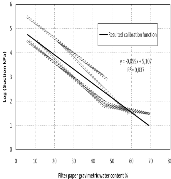
Figure 3. Resulted calibration function from the seven evaluated calibration curves for Whatman 42 filter paper
