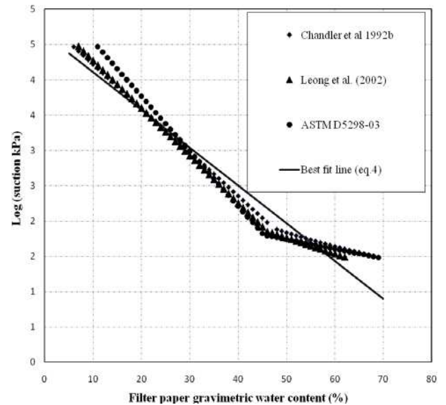
Figure 4. Best fit line resulted from the three evaluated calibration curves for Whatman 42 filter paper
