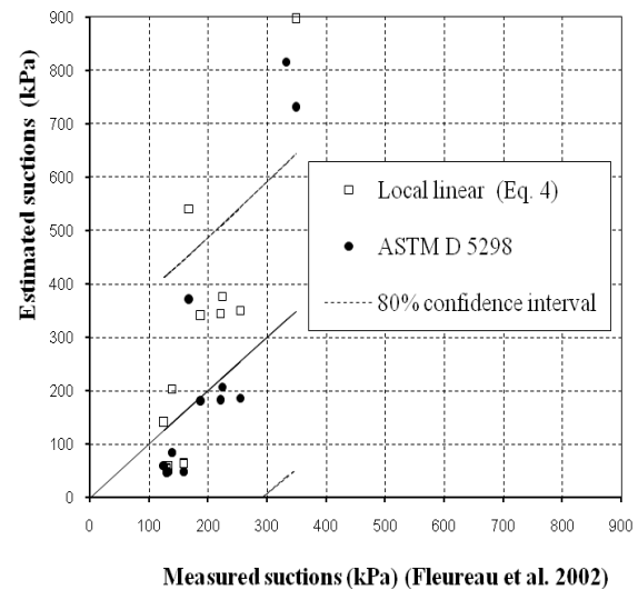
Figure 5. A pair of 80% confidence intervals (upper and lower limits) calculated from Eq (4) and ASTM calibration function
