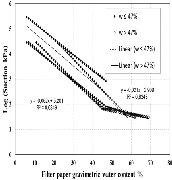
Figure 2. Two linear calibration functions resulted from the seven evaluated calibration curves for Whatman 42 filter paper
