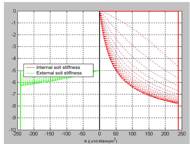
Figure 4. Soil stiffness decay during iteration, represented along the concrete wall, passive and active sides
