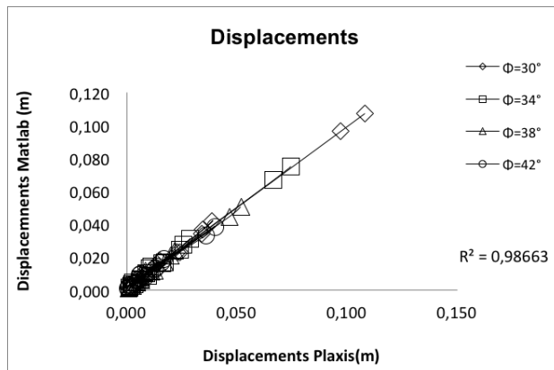
Figure 9. Displacements calculated for all excavation phases with the two wall stiffnesses and friction angles of 30 °, 34 °, 38 ° and 42 °
