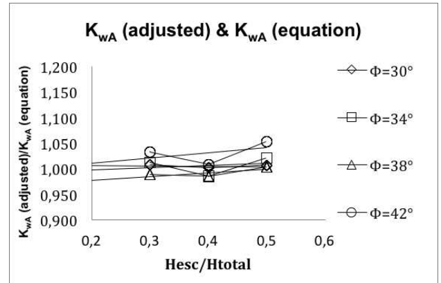
Figure 7. K_{WA}(\text{adjusted}) and by K_{WA}(\text{equation}) coefficients
