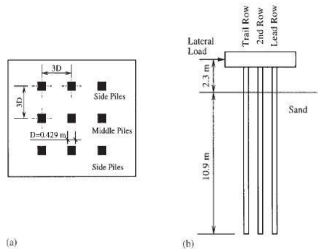
Figure 1. Layout of 3×3 pile group: (a) top view, (b) side view
