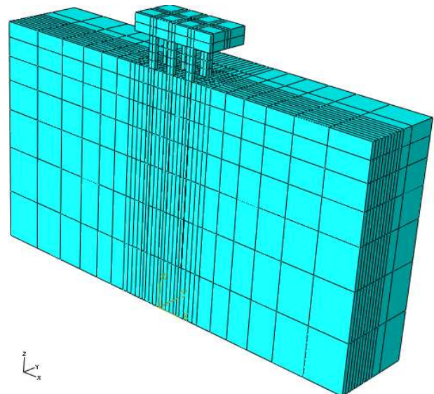
Figure 2. Finite element mesh for 3×3 pile group with cap
