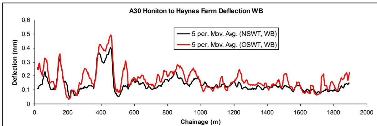
Figure 3. Deflection profiles for NSWT and OSWT in the WB direction
