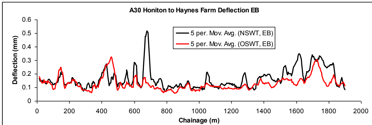
Figure 2. Deflection profiles for NSWT and OSWT in the EB direction
