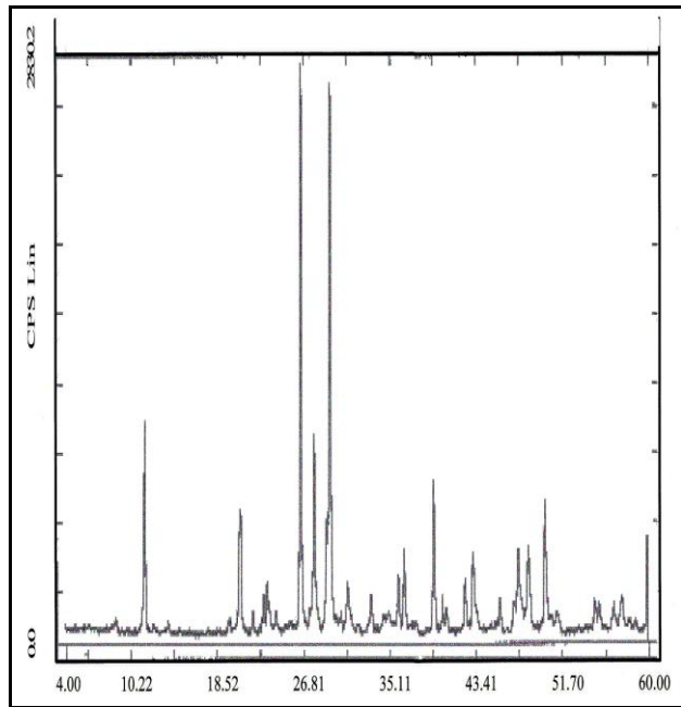
Figure. 2. XRD pattern of silty sand soil.
